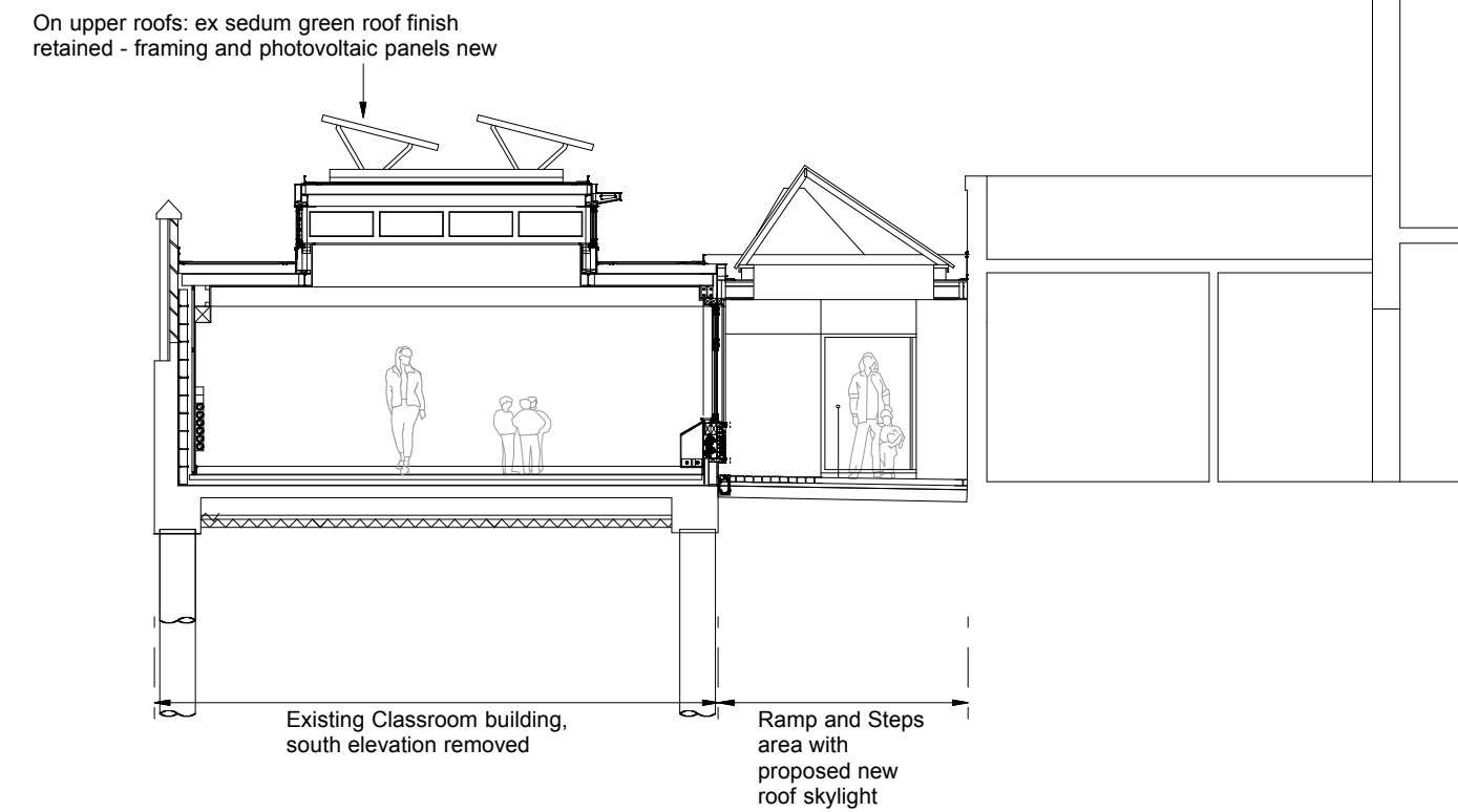
Section BB: Classroom & "Link" area
