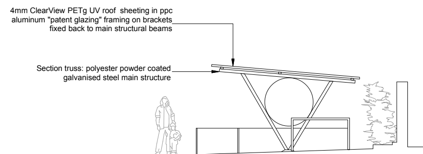
Section CC: New Cycle & scooter shelter area
