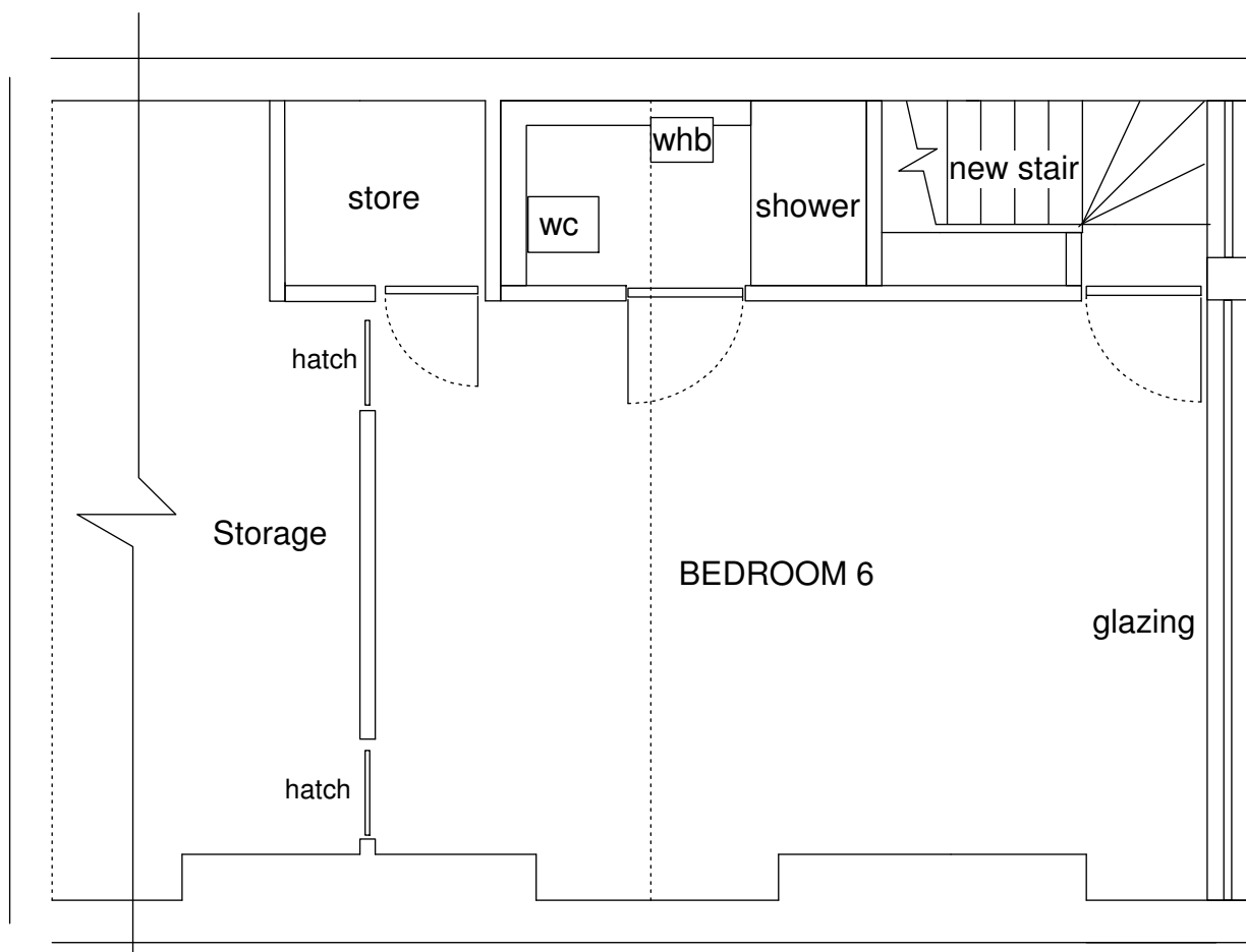
Third Floor as Proposed
