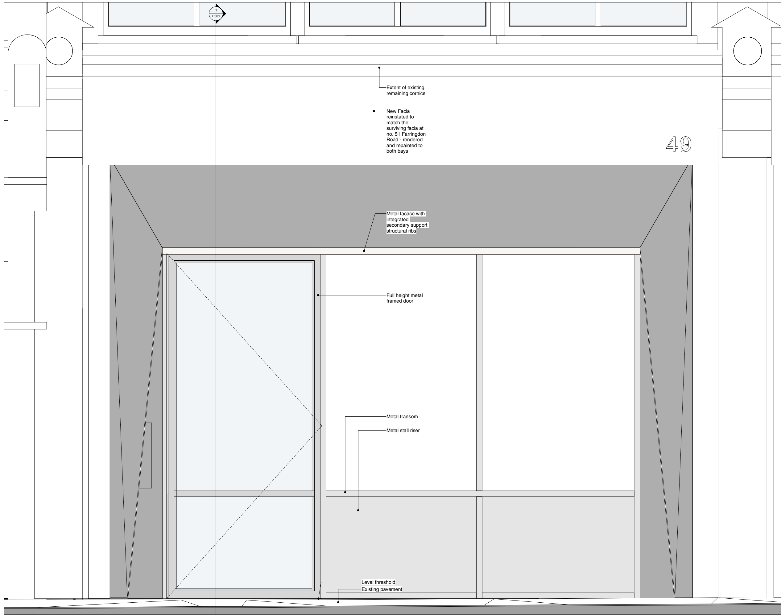
P302 Typical Shopfront Elevation Bay
