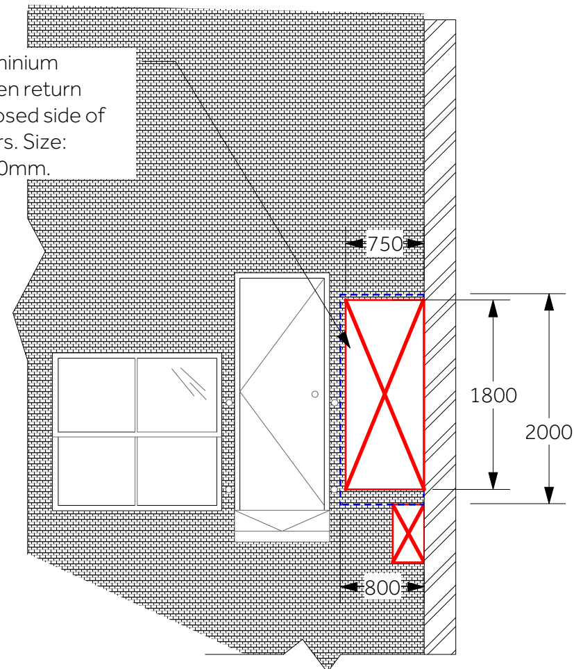
Elevation B Condensor unit Elevation - scale 1:50
