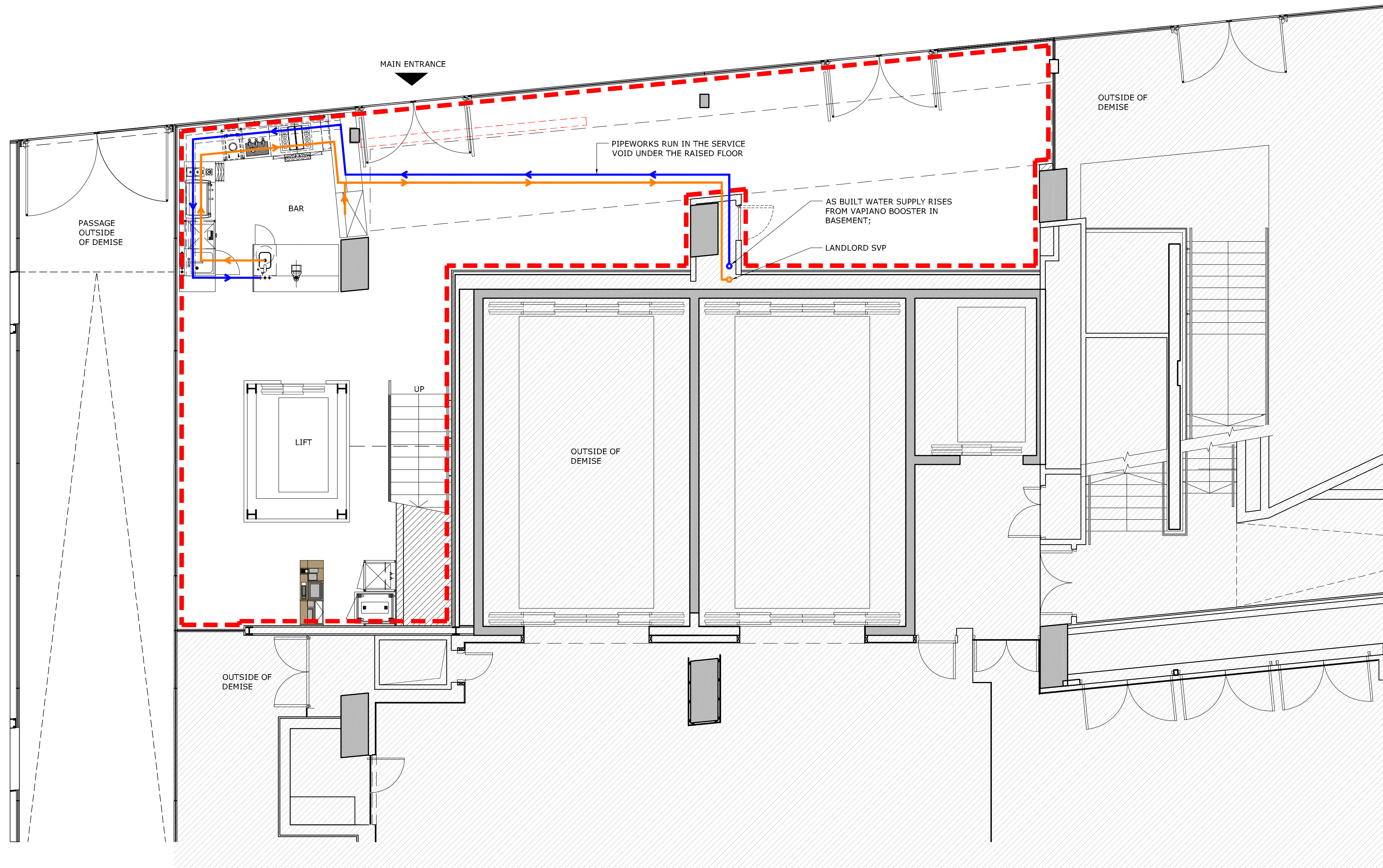
1 PROPOSED GROUND FLOOR PLAN 1:50 @ A1
