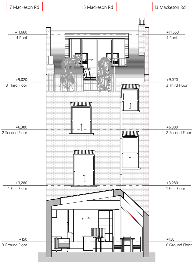
Section AA 1:100
