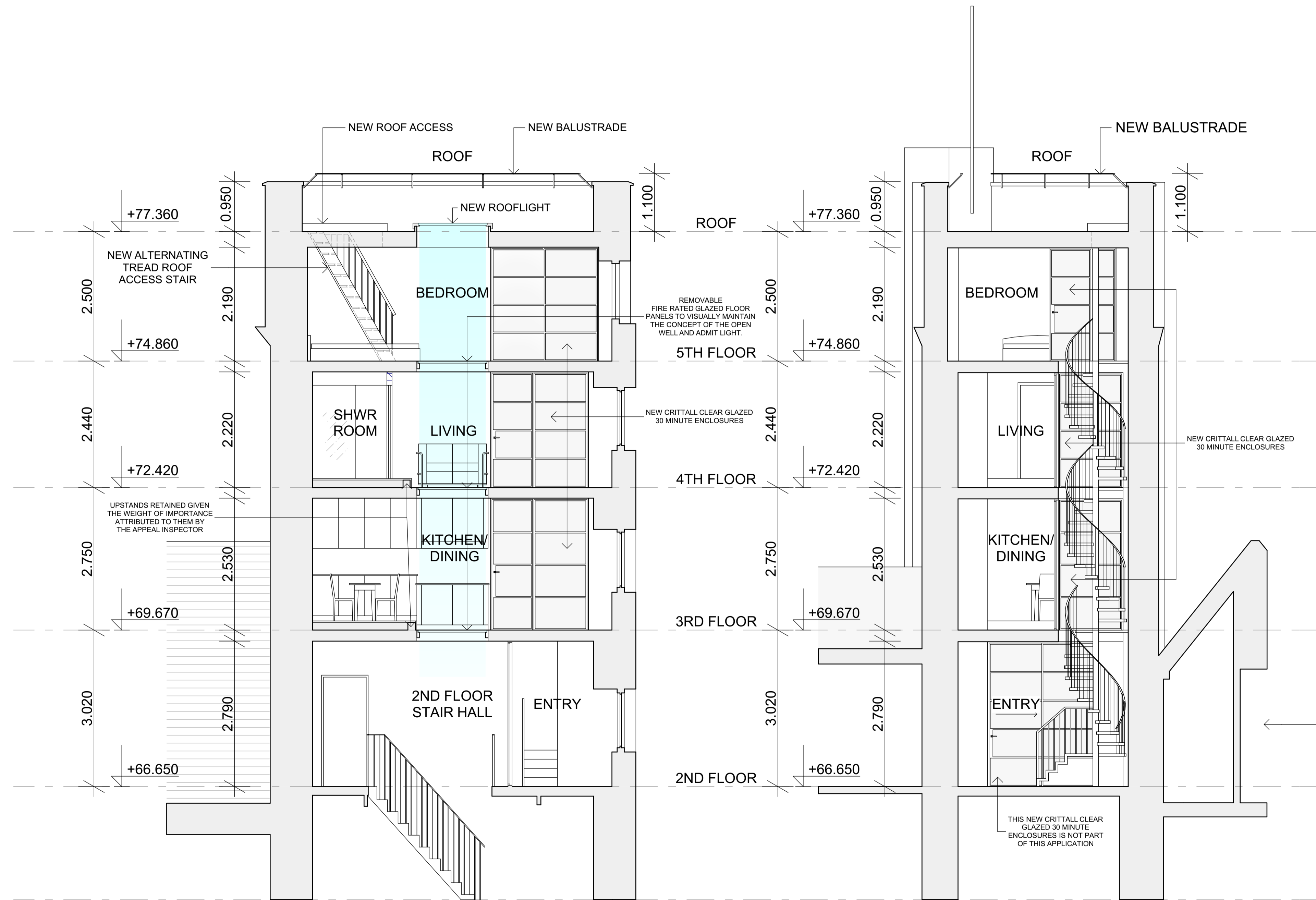
TOWER SECTION A - A 1:50
