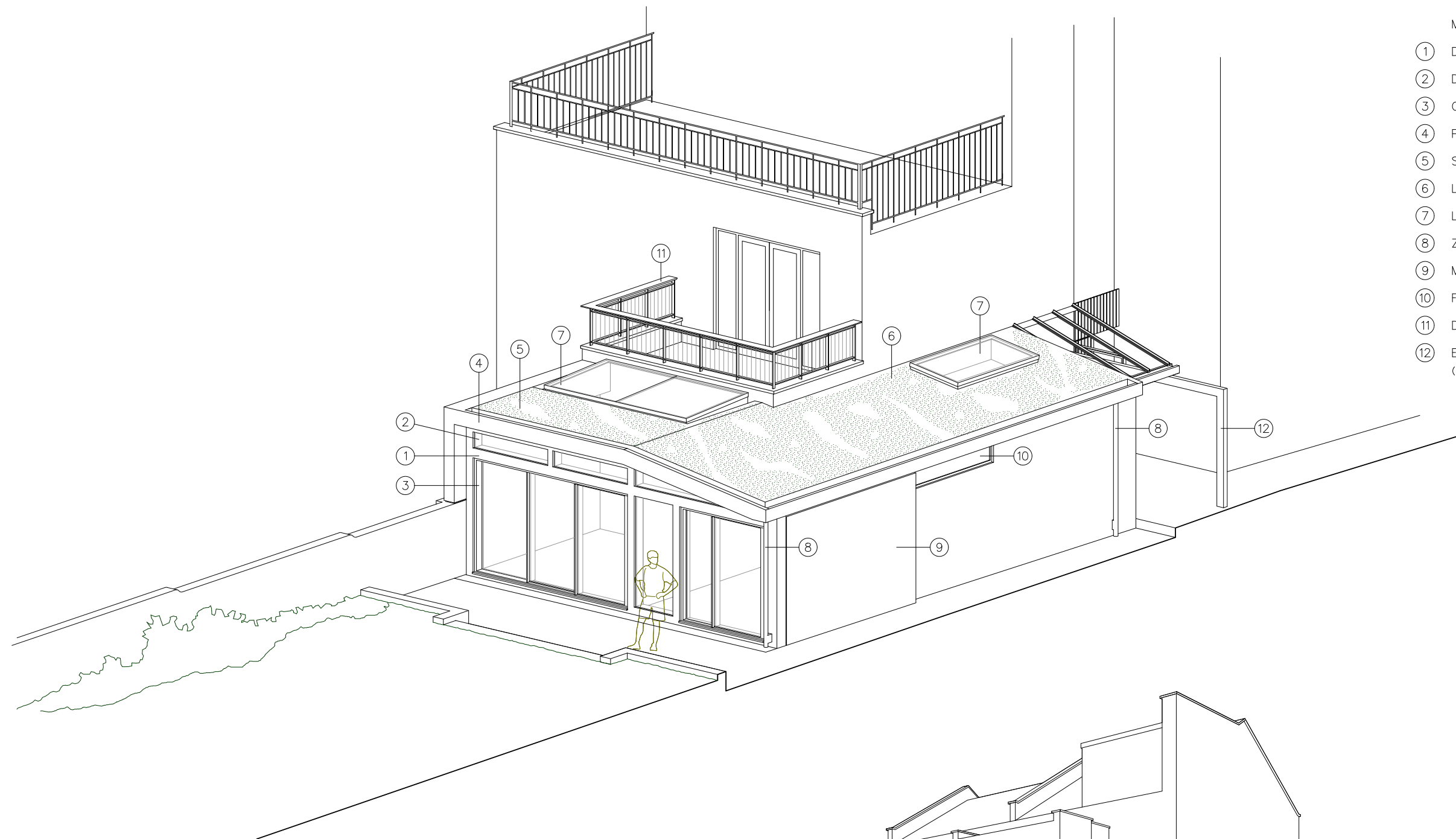
1. AXONOMETRIC VIEW
