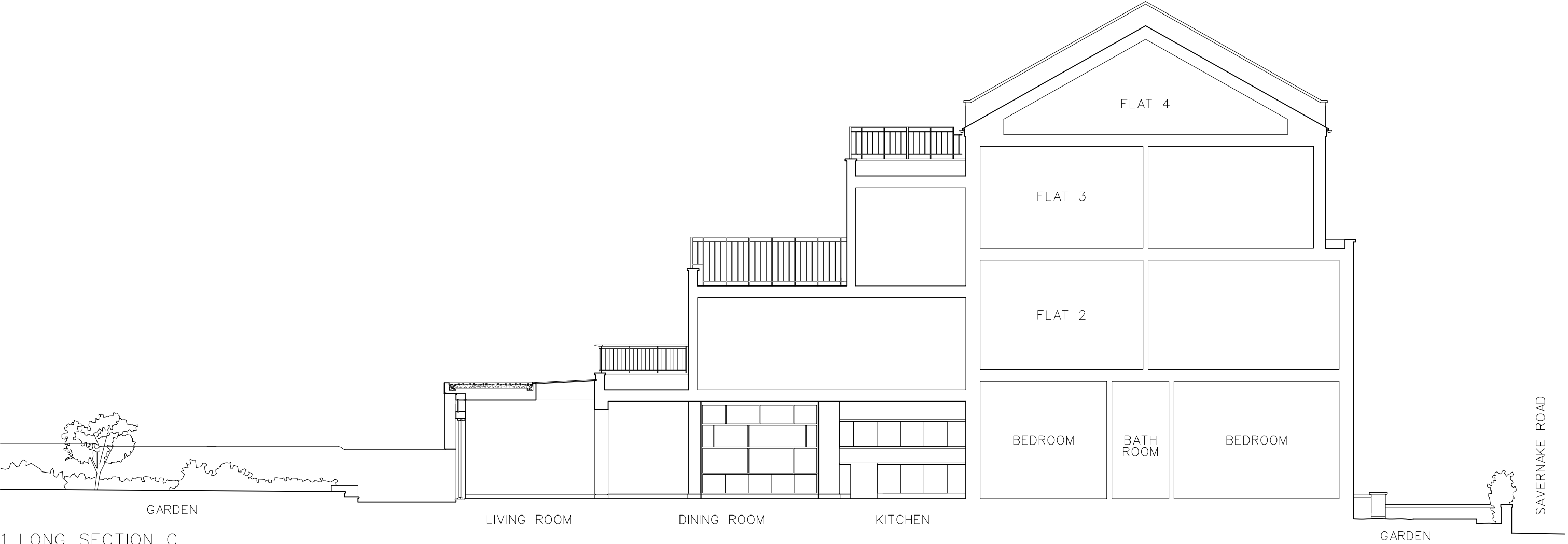
1. LONG SECTION C
