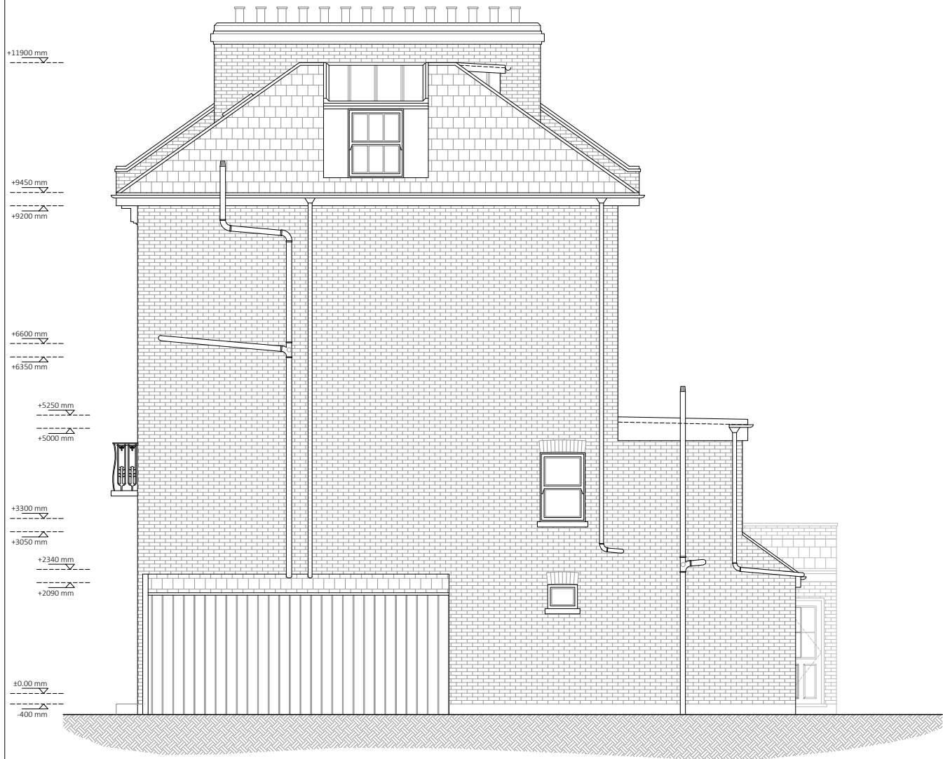
EXISTING WEST SIDE ELEVATION
