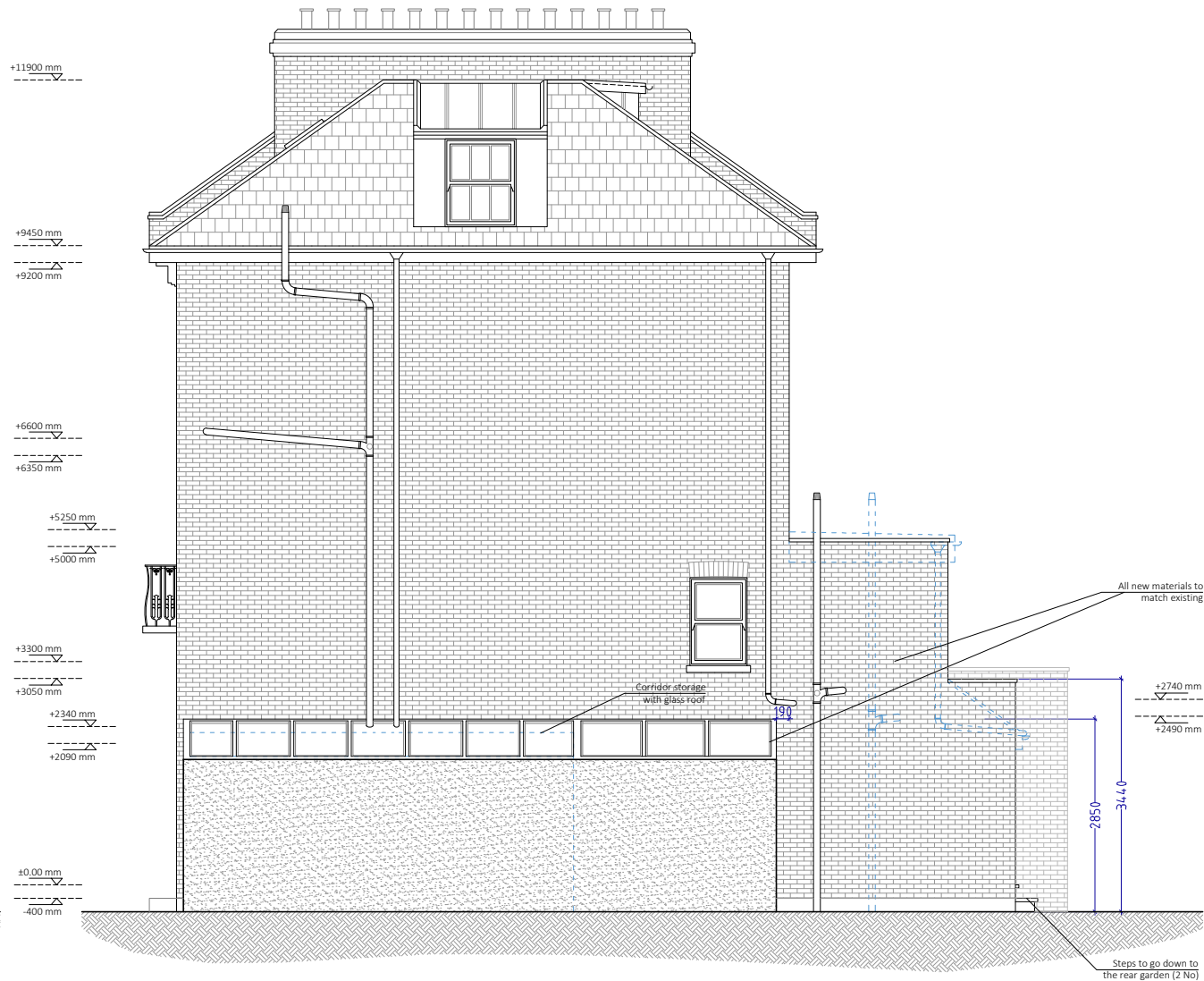
PROPOSED WEST SIDE ELEVATION
