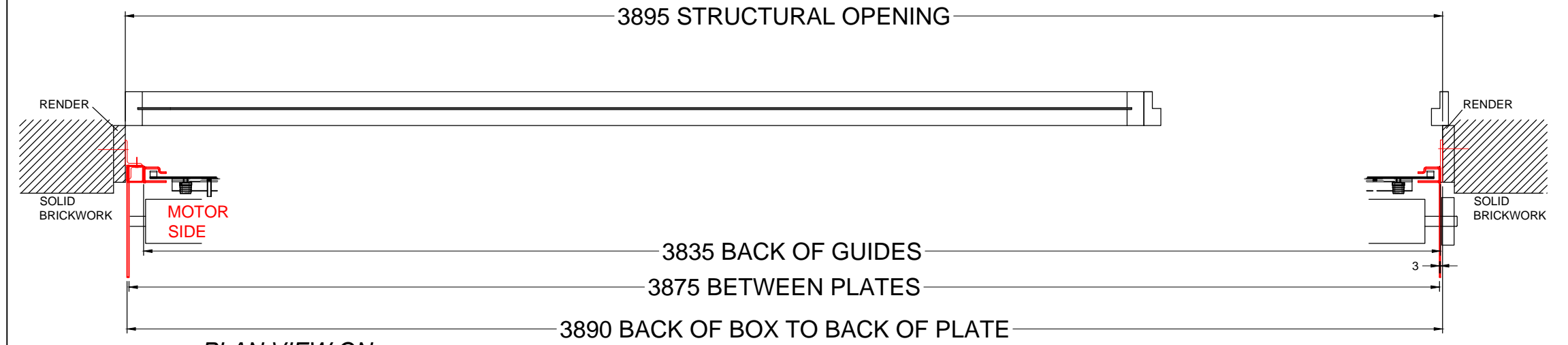
PLAN VIEW ON ROLLER SHUTTER
