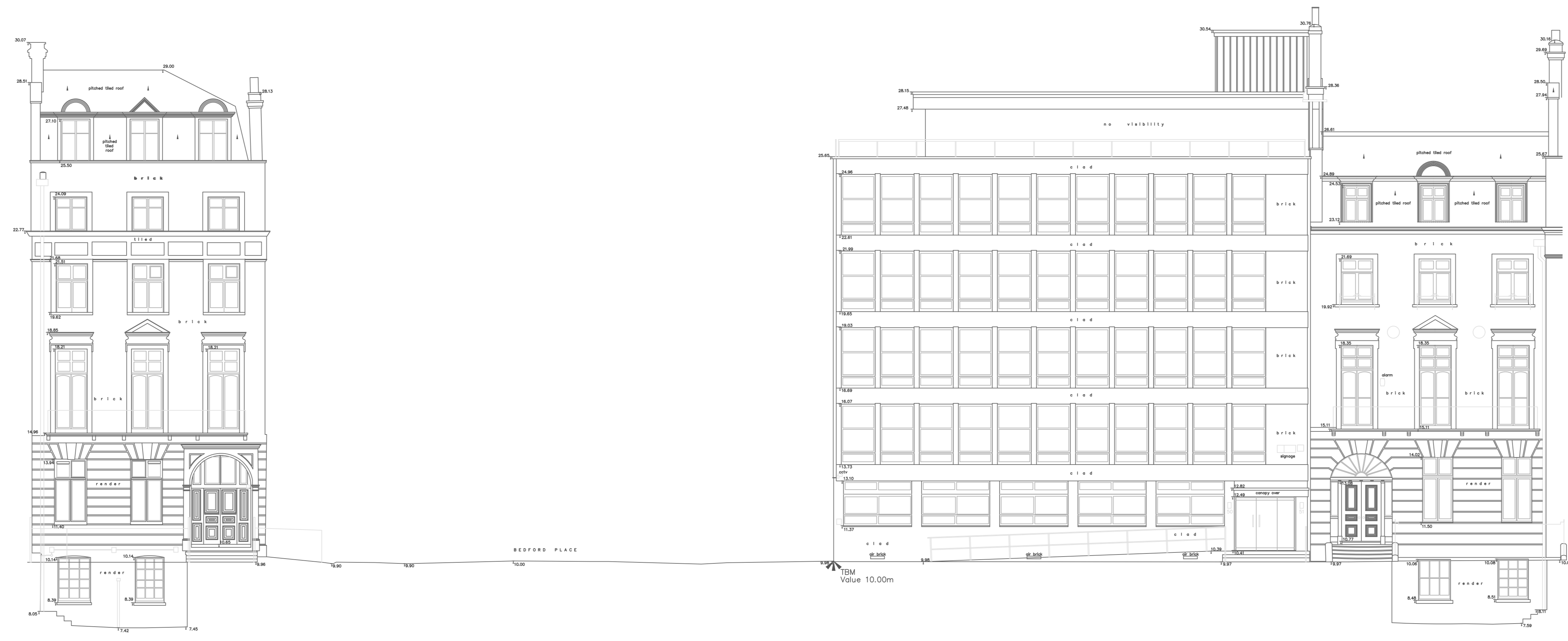
ELEVATION FRONT
