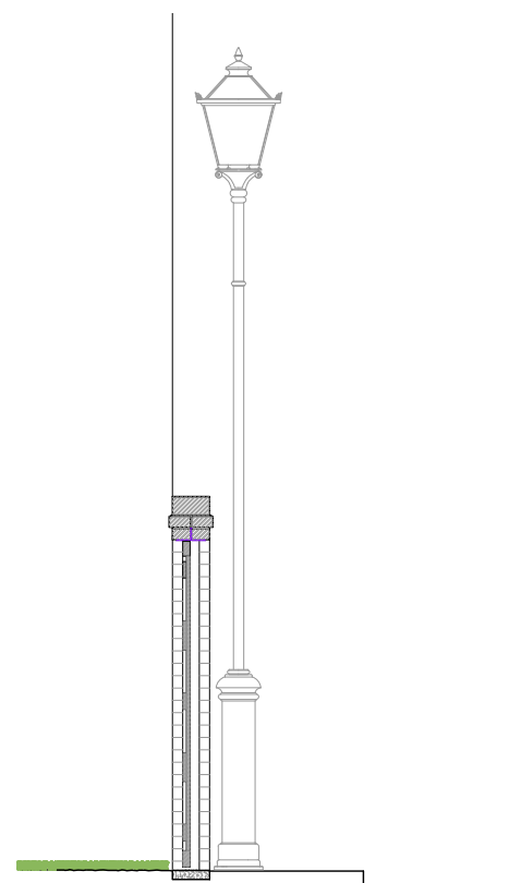
02. SECTION @1:50
