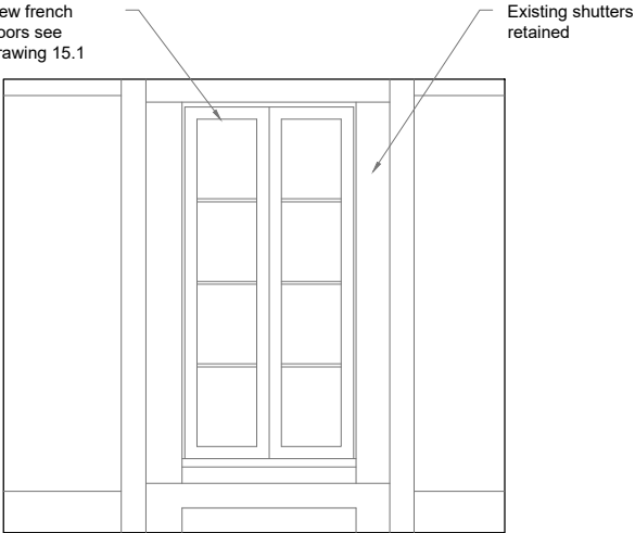
Proposed_UG03.0 LIBRARY Elevation A
