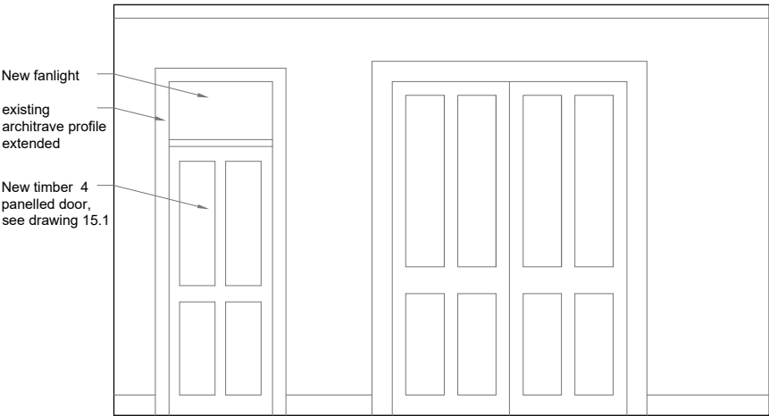
Proposed_F04.0 BEDROOM Elevation A
