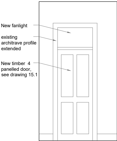
Proposed_F04.0 HALL Elevation C
