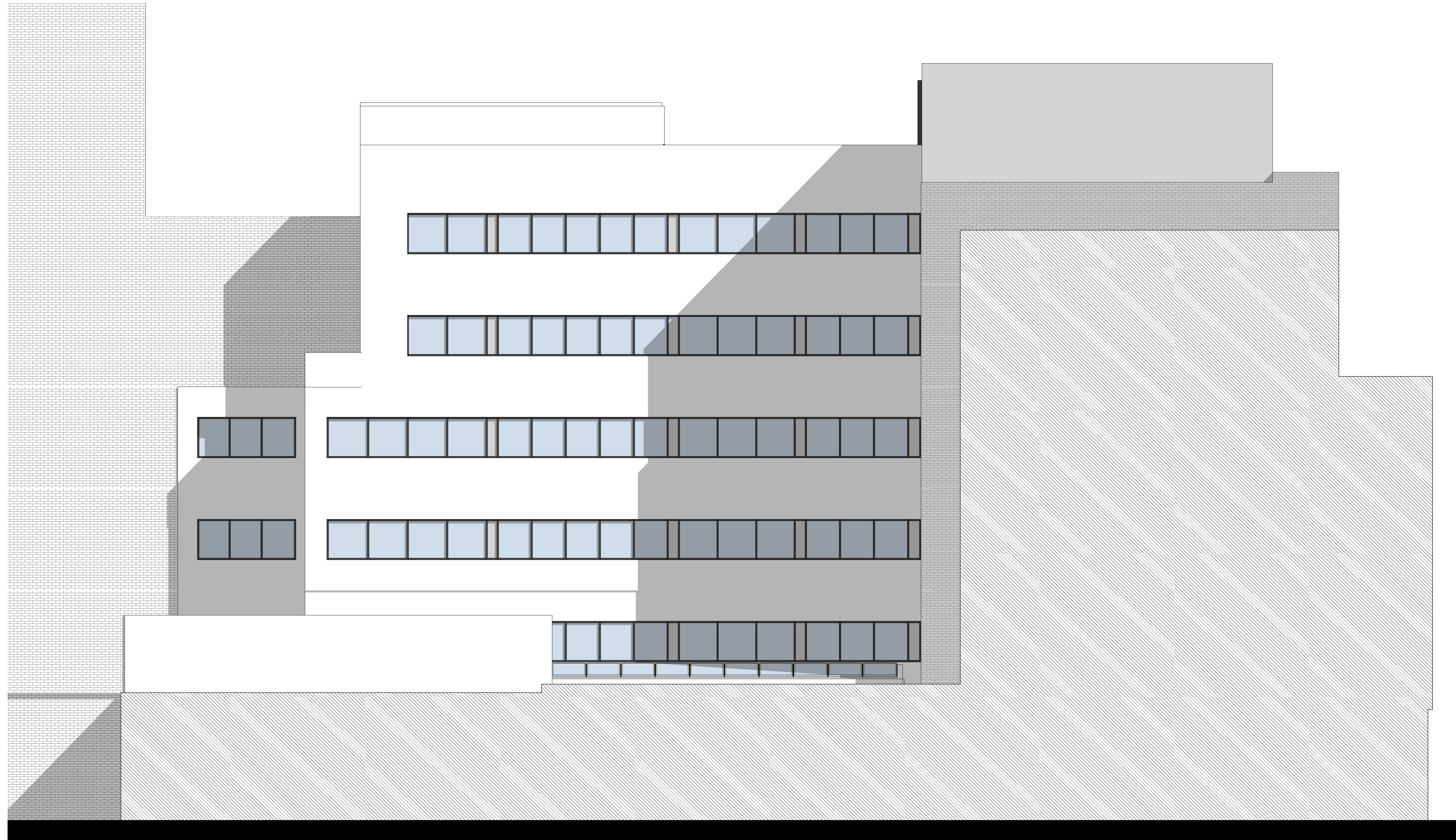
2 Existing South Elevation 1:50
