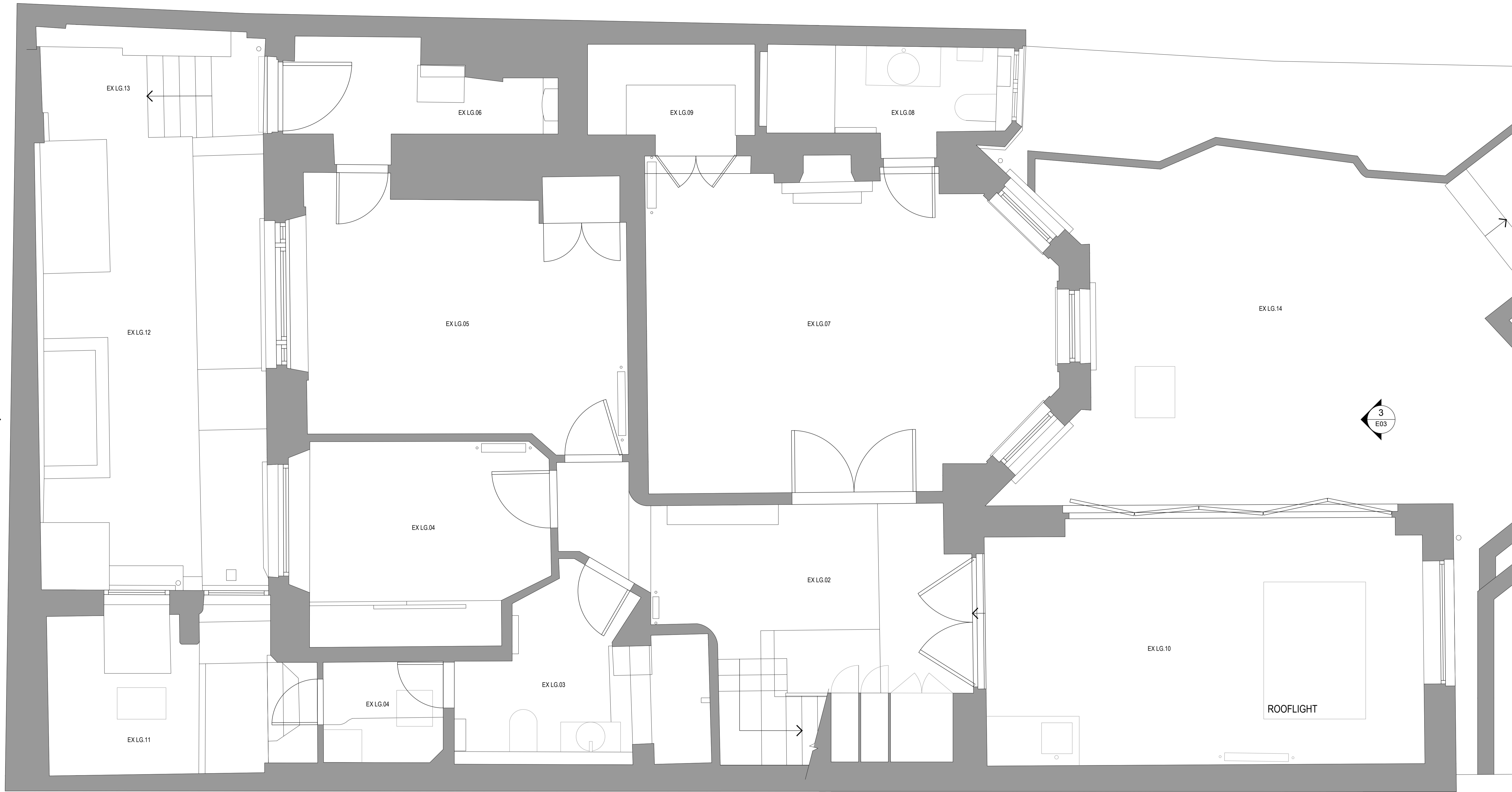
1 EXISTING - GROUND ROOF PLAN SCALE: 1:50 @ A1 / 1:100 @ A3
