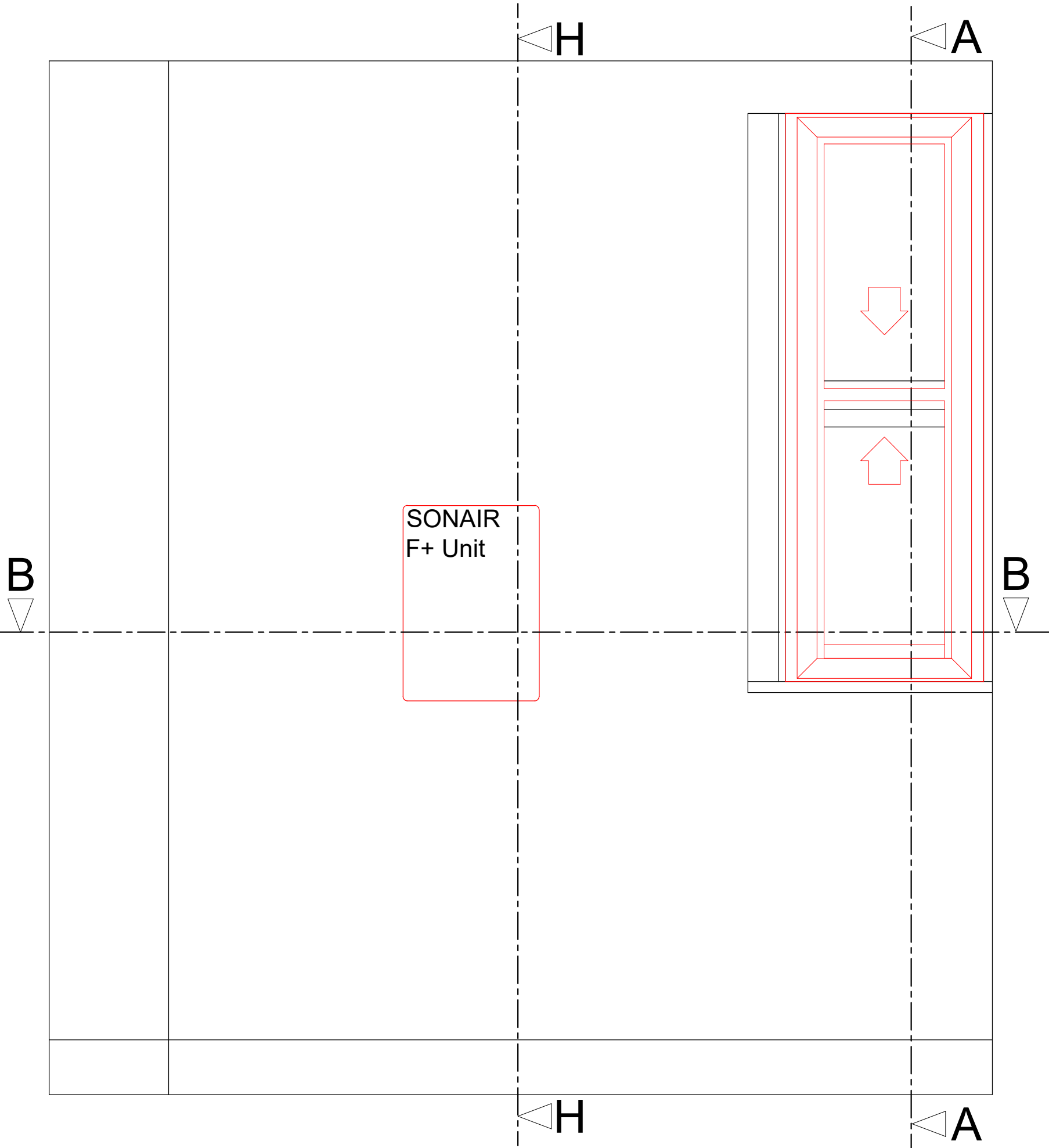
Internal Room Elevation with Secondary Glazing Installed Scale: 1:10
