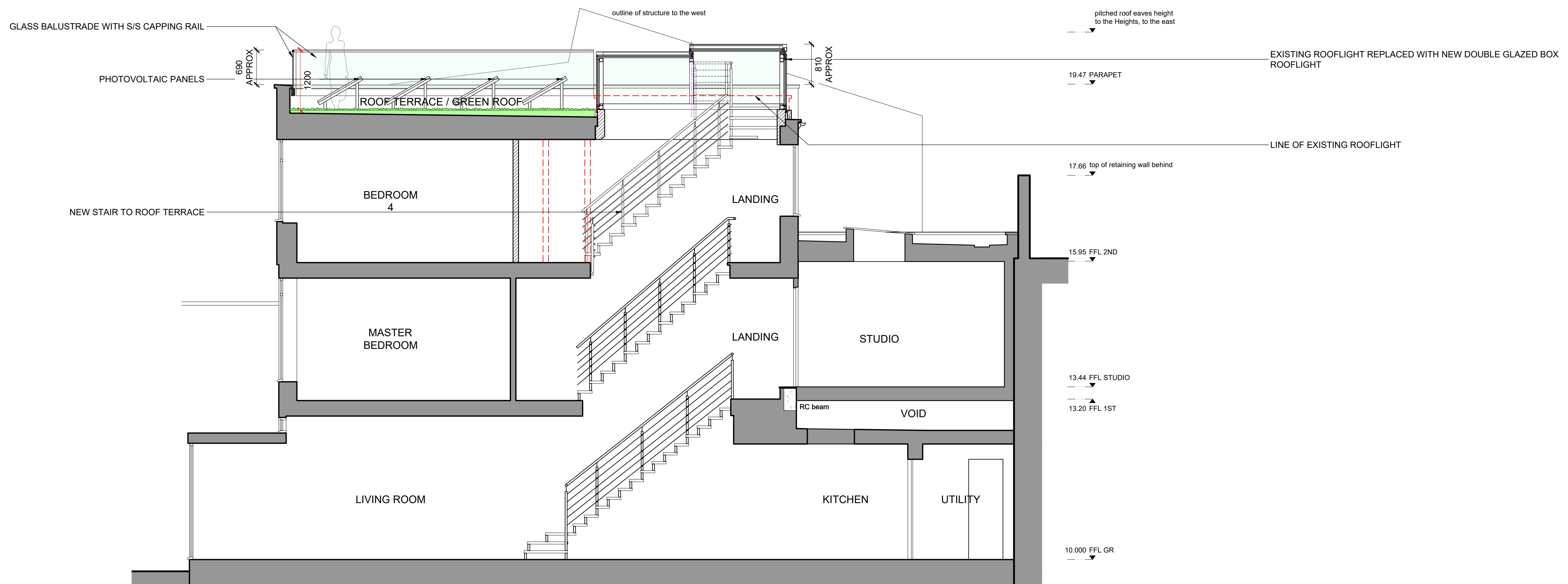
2 PROPOSED SECTION BB
