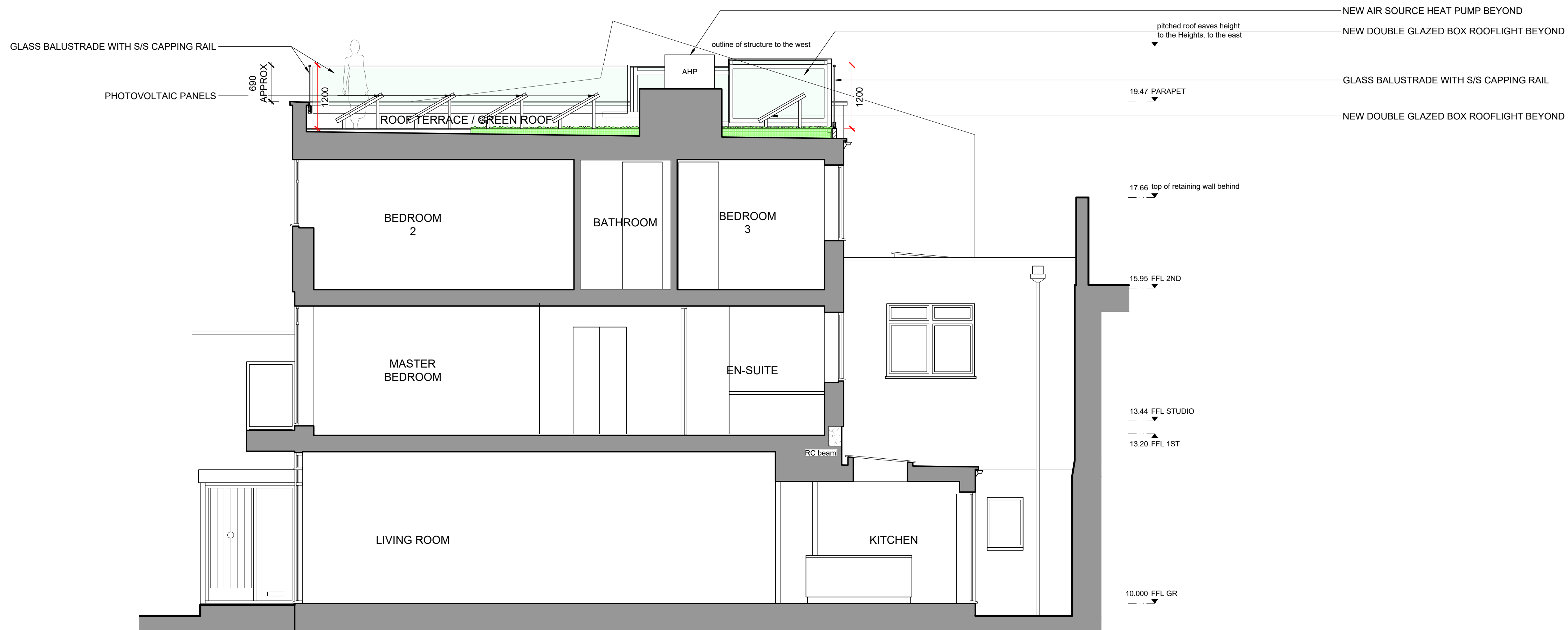
1 PROPOSED SECTION AA
