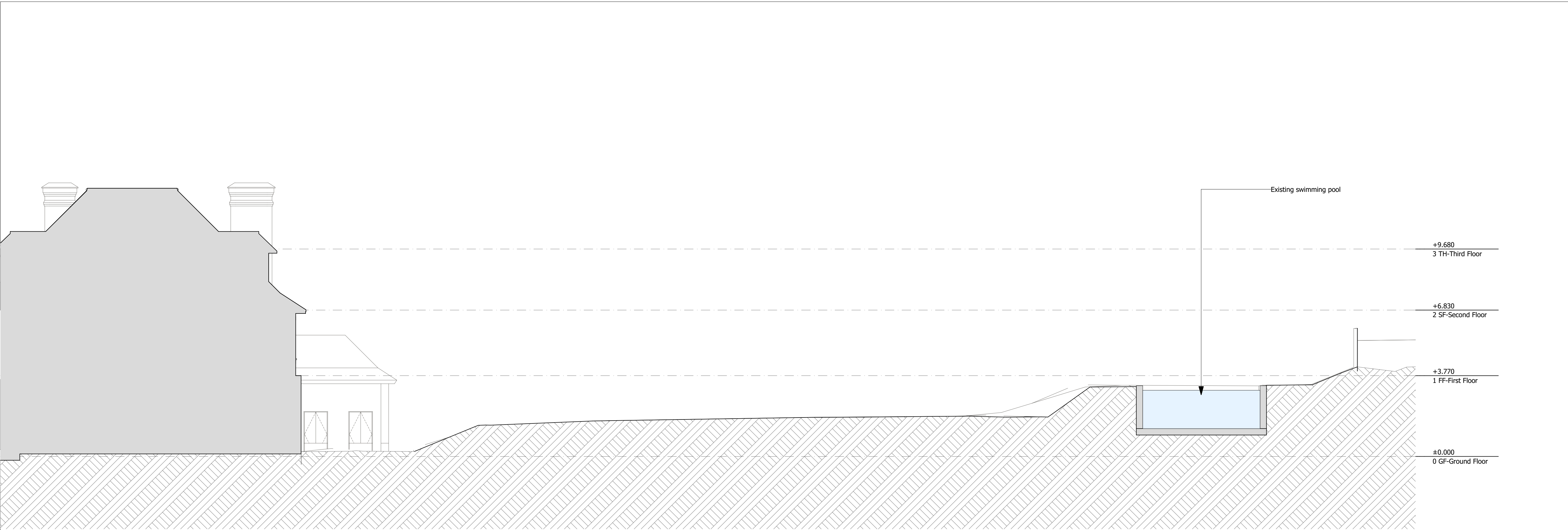
B Section - Existing 1:100
