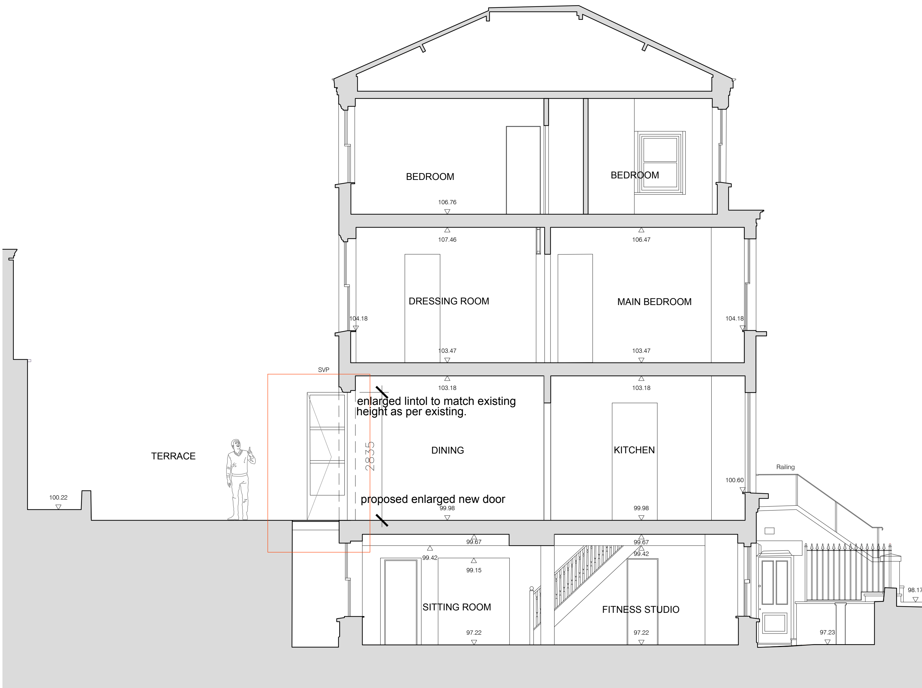
SECTION AA
