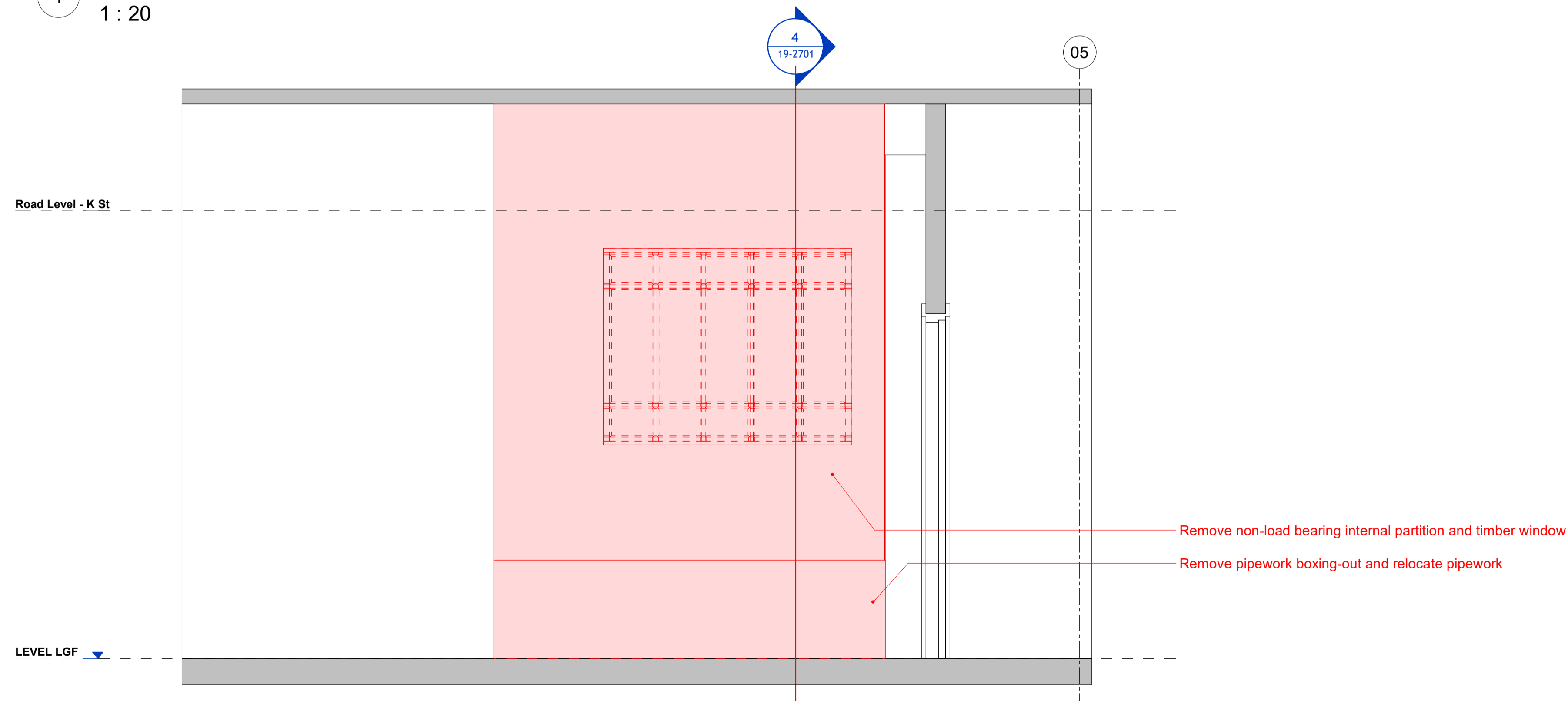
2 Existing Elevation of LG43a from LG35a 1 : 20
