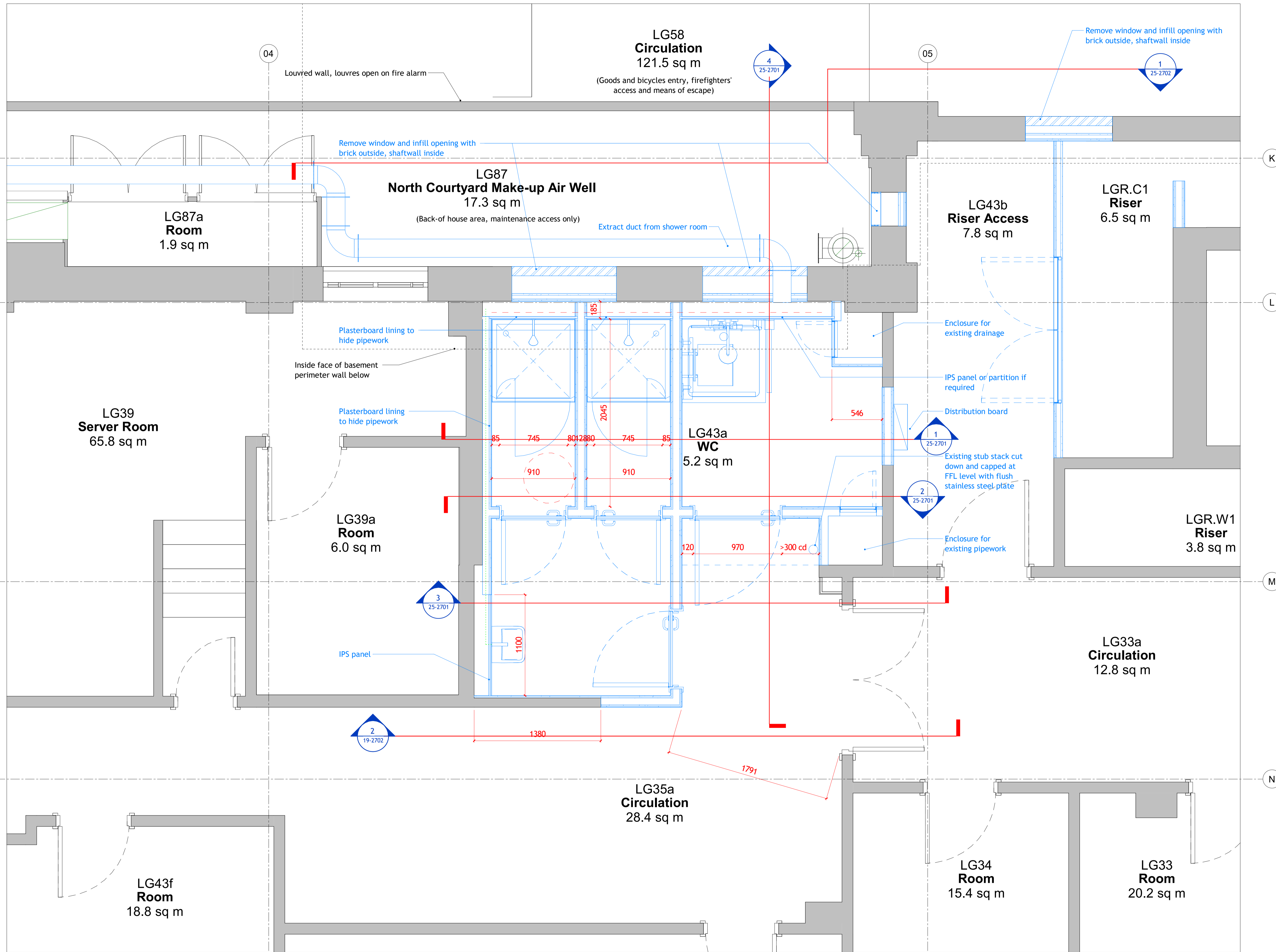
1 Proposed Plan - LG43a Shower Room 1 : 20
