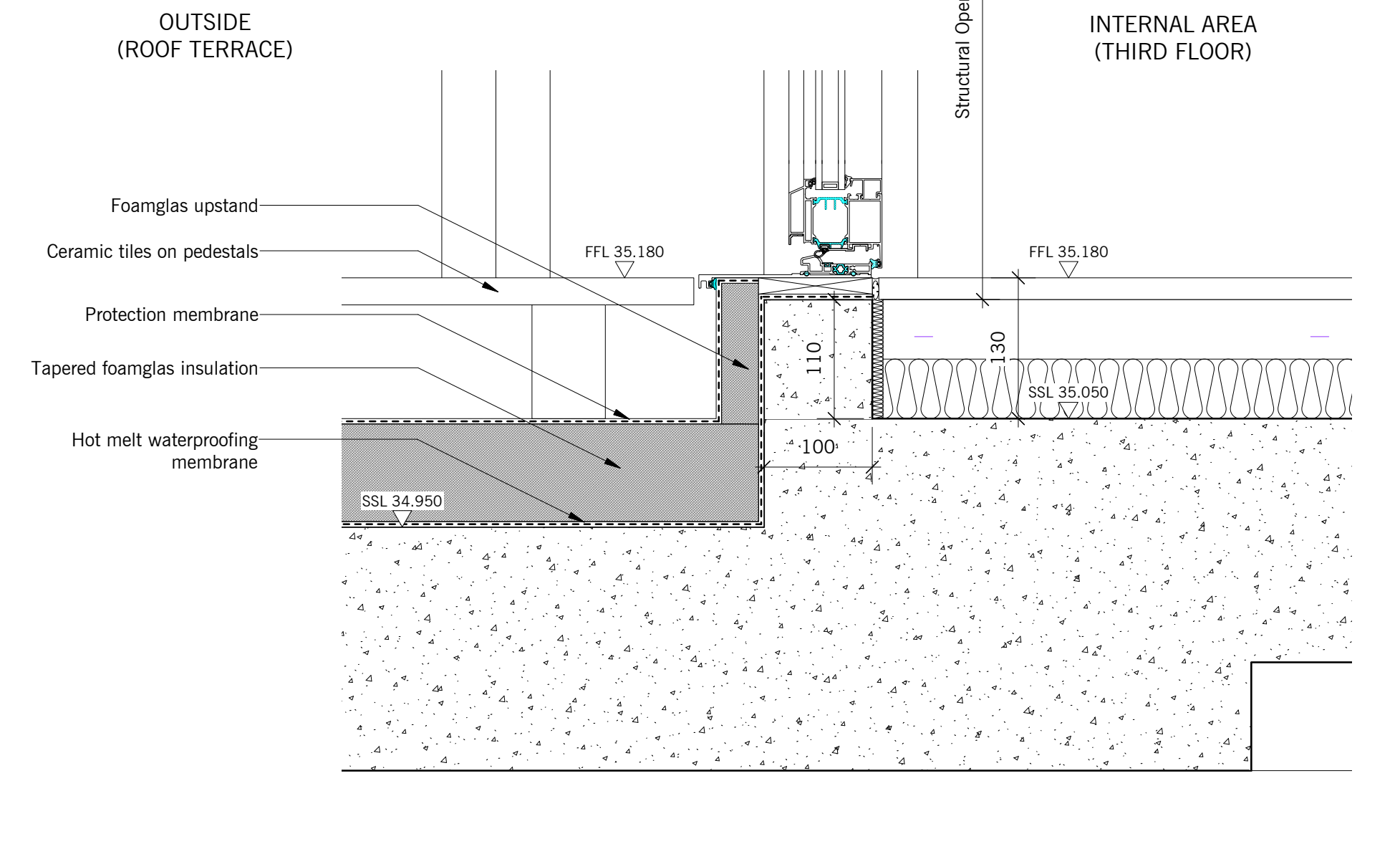
1 WINDW CILL DETAIL SCALE 1:5
