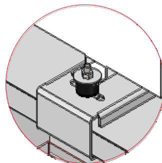
DETAIL A ANTI VIBRATION MOUNT FITTING REF: TCSB-90-9011-EN SCALE 1:5
