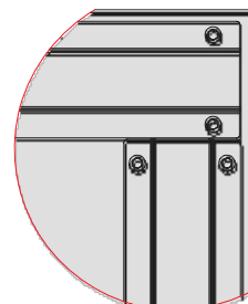
DETAIL B HIGH TORQUE FIXINGS REF: TCSB-85-8511-EN SCALE 1:7
