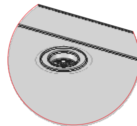
DETAIL C CONDENSATE R/ANGLED DRAIN FITTING REF: TCSB-95-9511-EN SCALE 1:5
