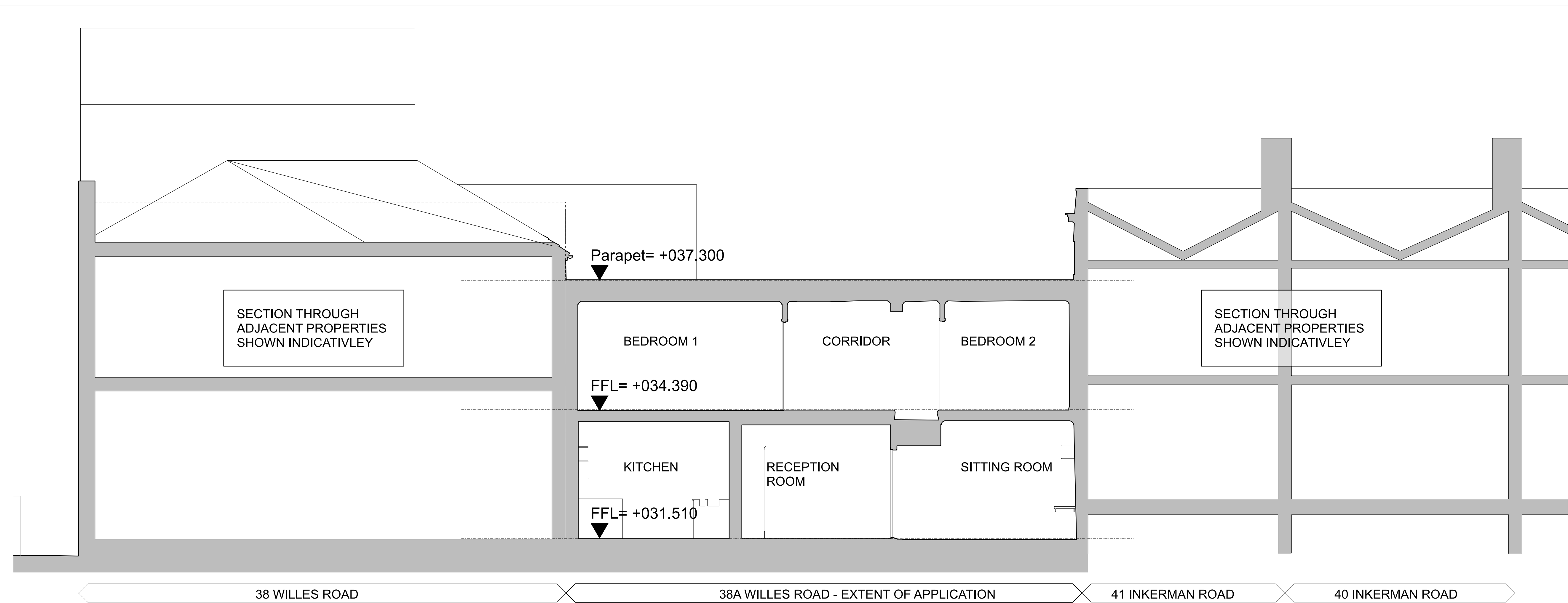
02 SECTION DD: EXISTING LONG SECTION
