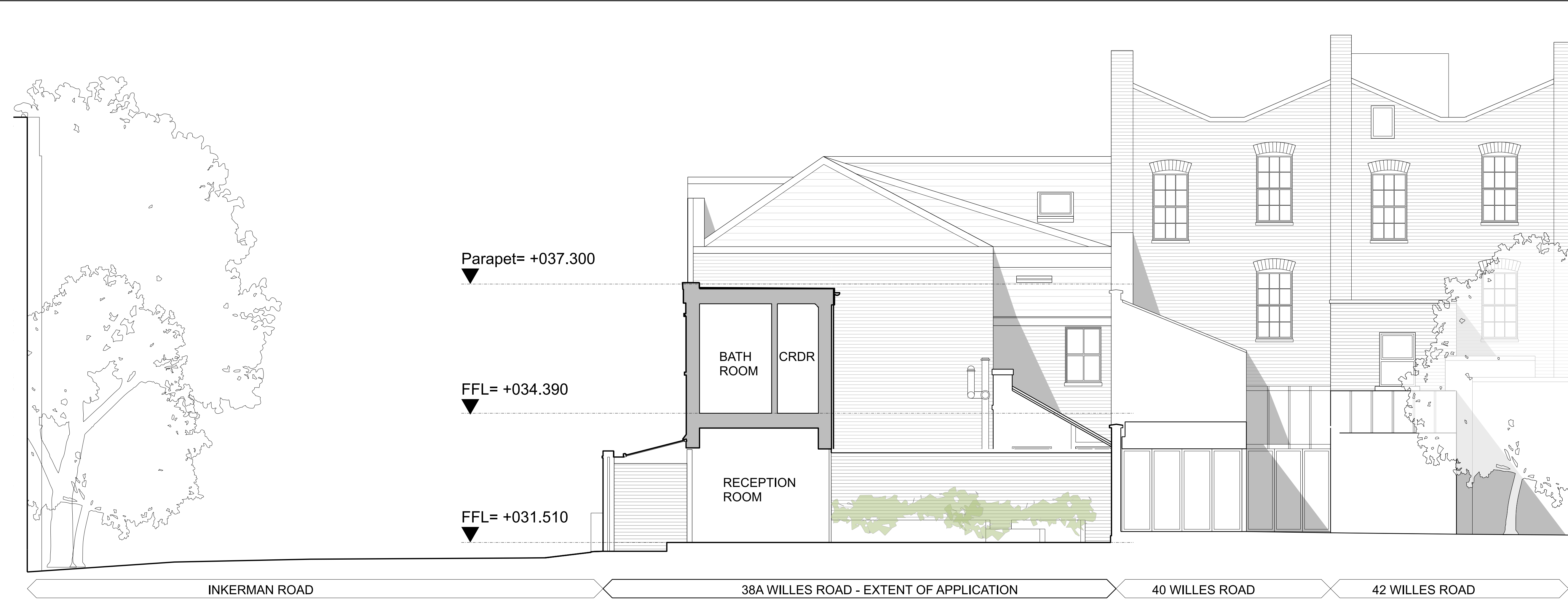
01 SECTION CC - SECTION THROUGH ENTRANCE
