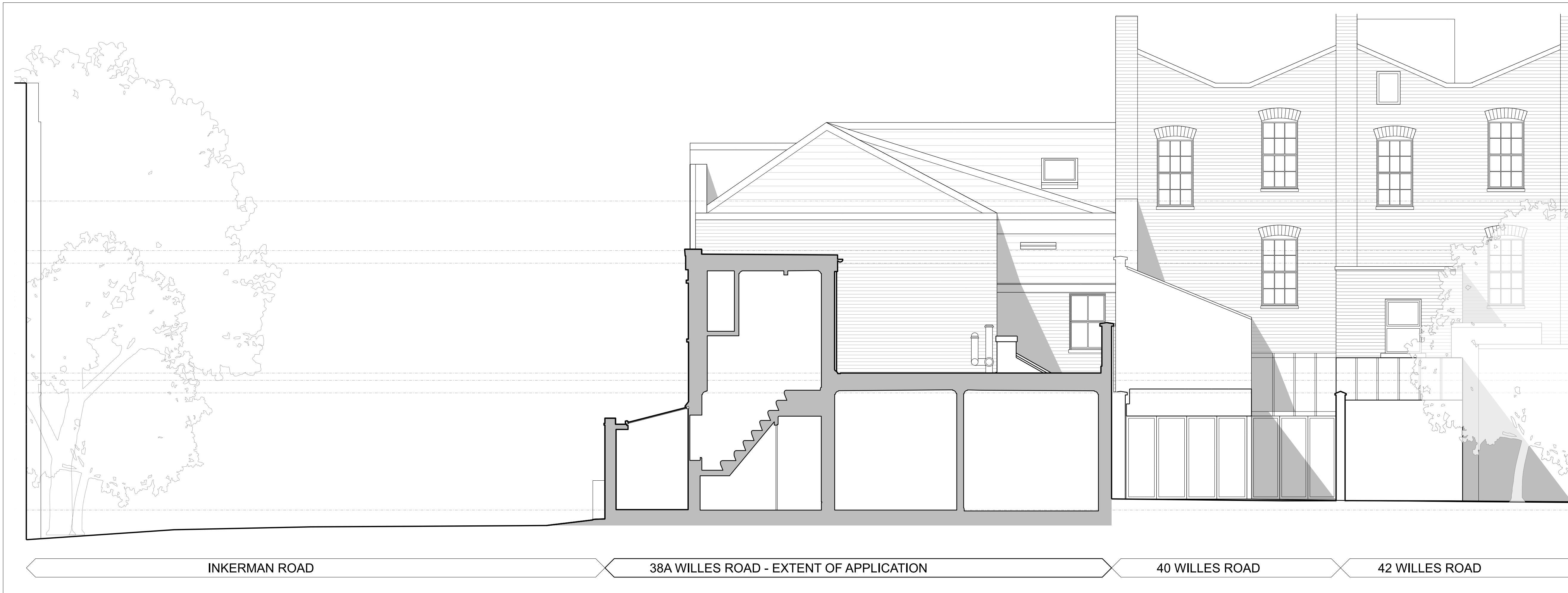
02 SECTION BB - THROUGH EXISTING BUILDING
