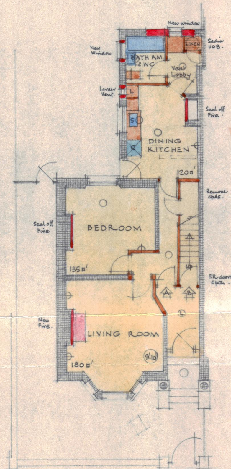
GROUND FLOOR
