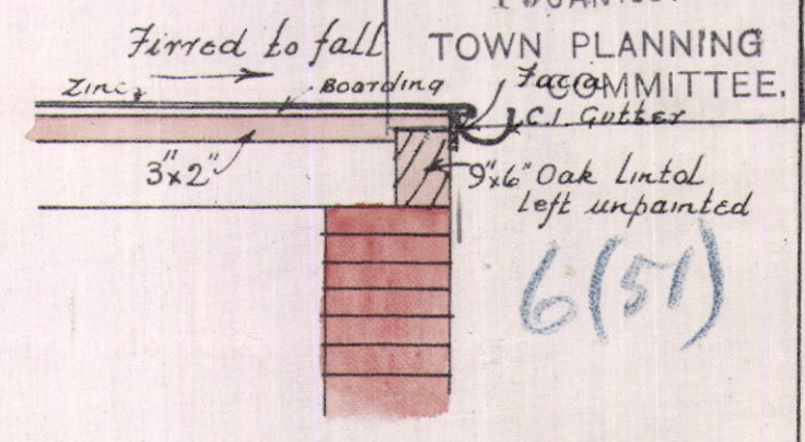
Half-inch detail.
