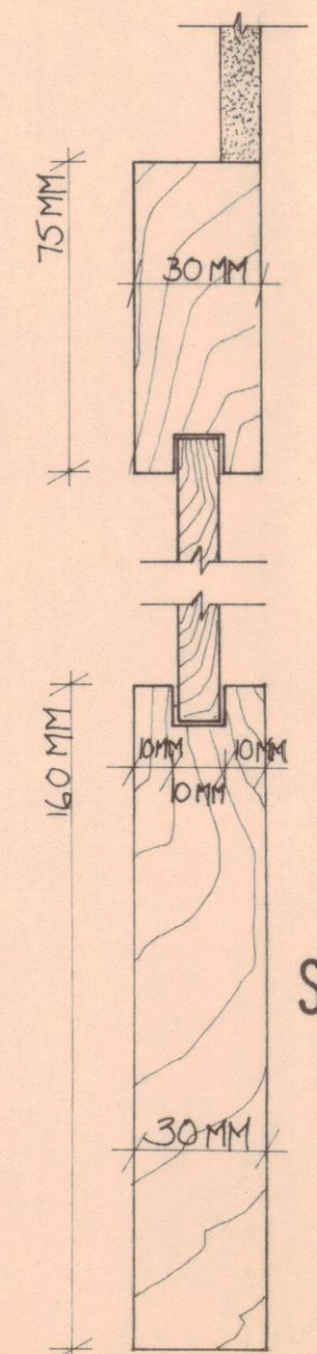
Panelling fixing 1:2
