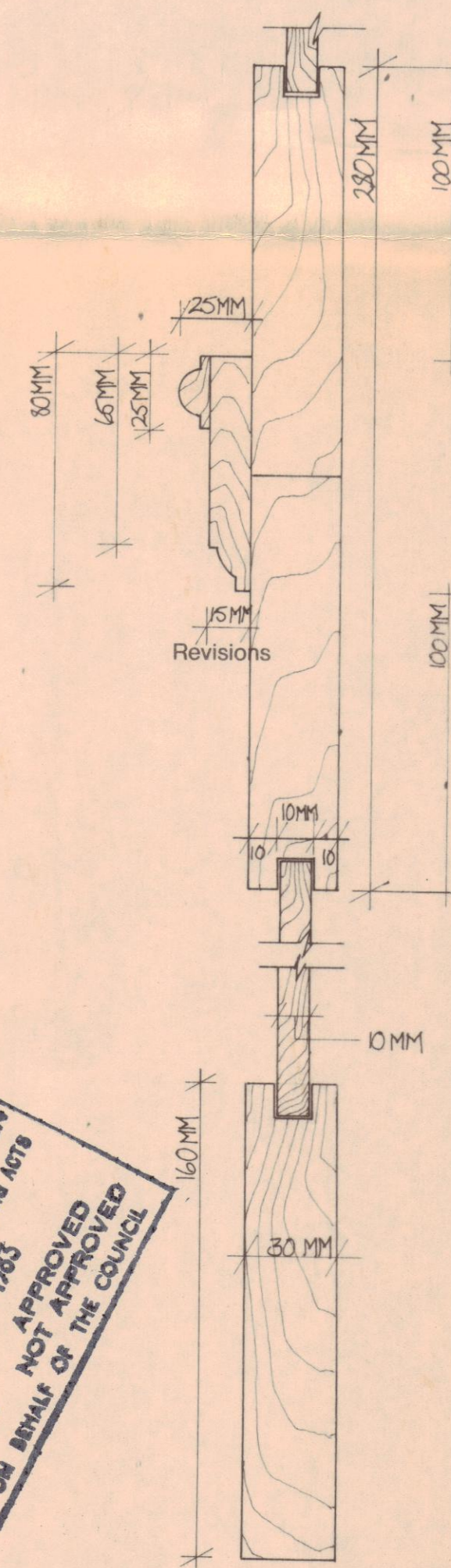
Skirting & Handrail detail 1:2
