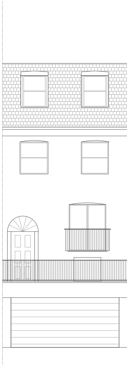
FRONT ELEVATION E: 1/100
