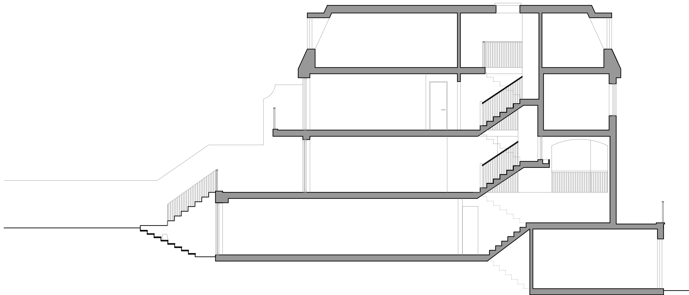
SECTION AA E: 1/100
