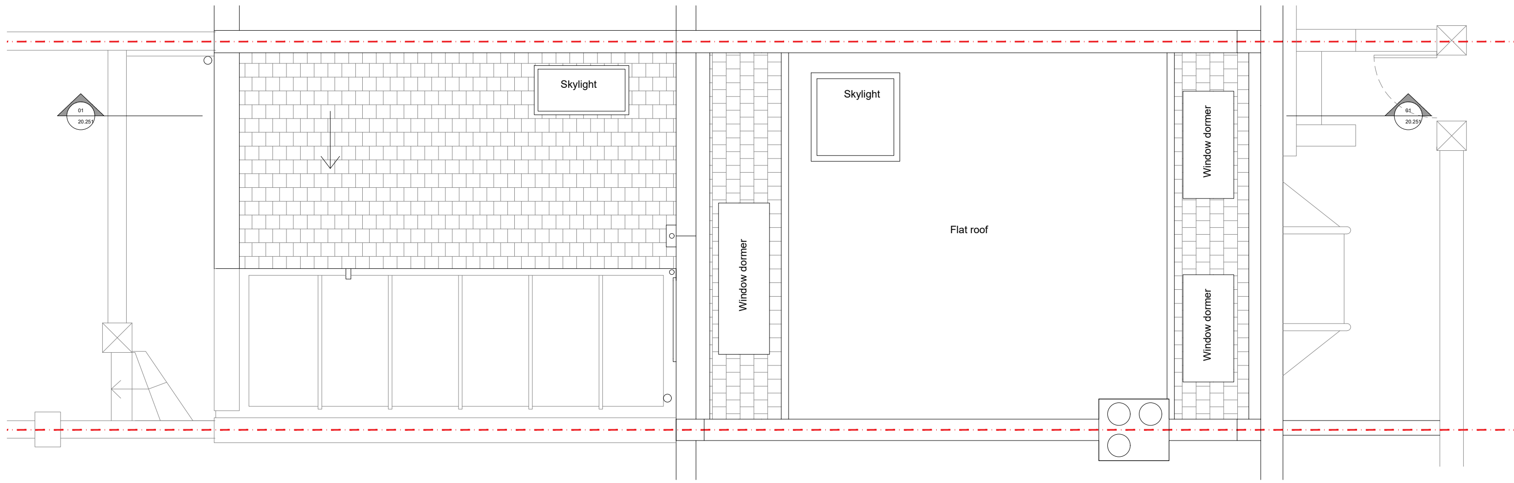
01 Proposed Mansard Plan Option 2 20.204 Scale 1:50 @ A3
