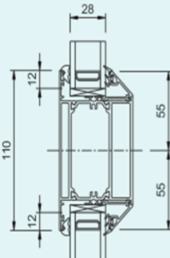
Midrail To align with a midrail in a door Section C - C
