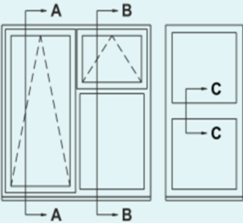
Midrail To align with a midrail in a door Section C - C
