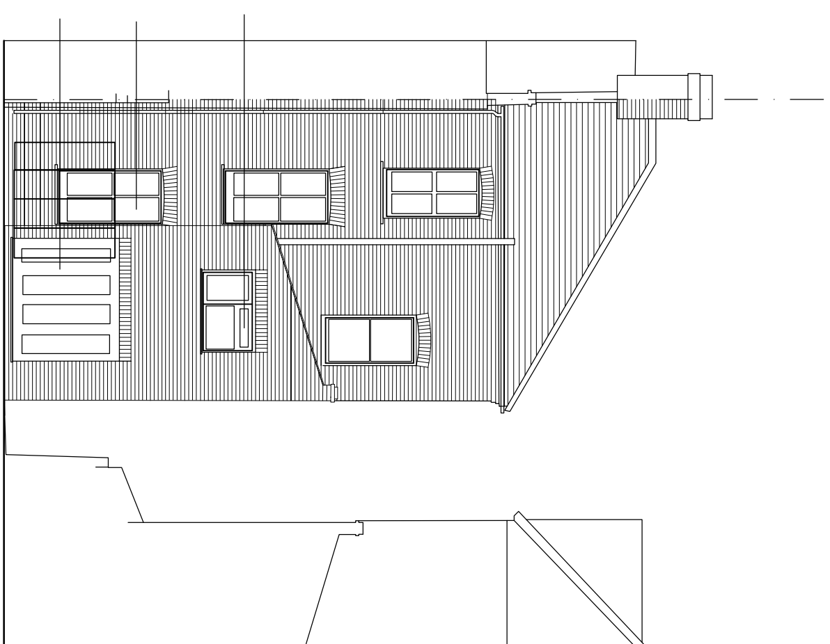
REAR ELEVATION
