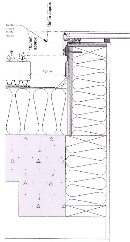
DETAIL AT EDGE OF R05 (see 468.506)
