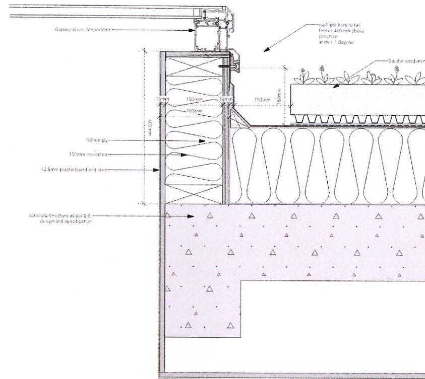
DETAIL AT EDGE OF ROOFLIGHT
