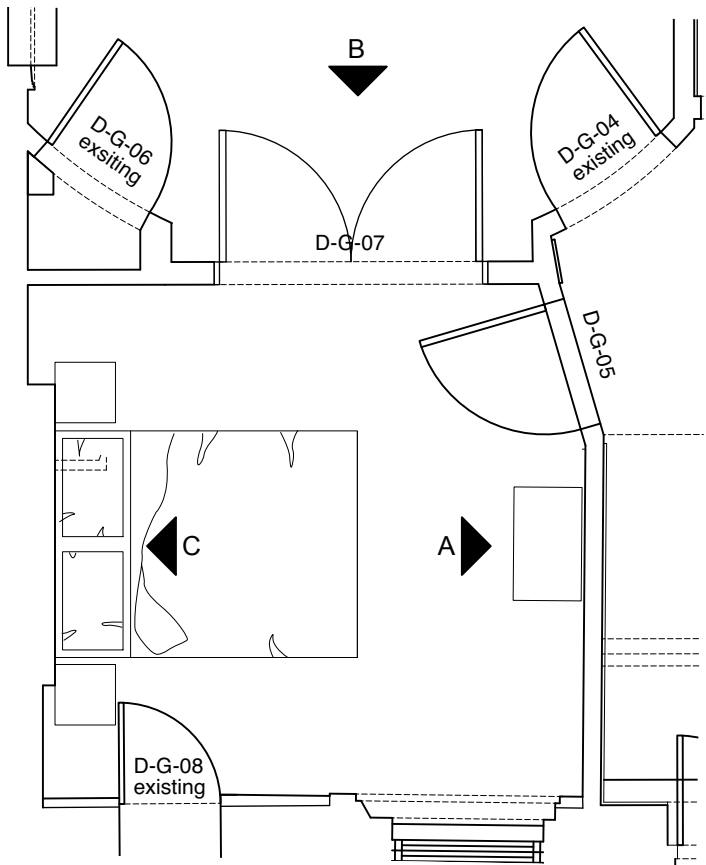
Proposed Plan
