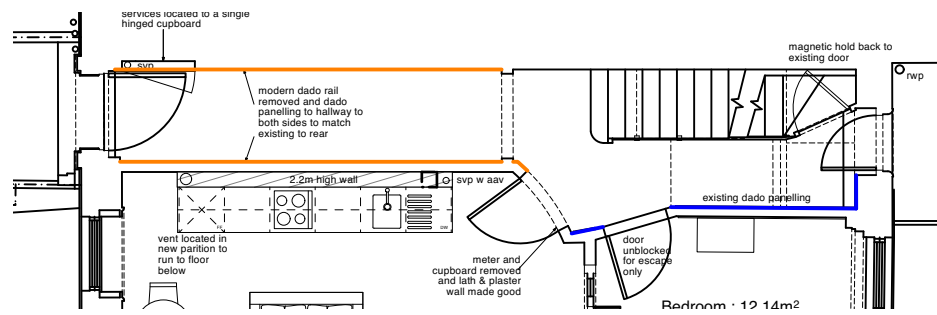
1:100 Location of panelling to Ground Floor
