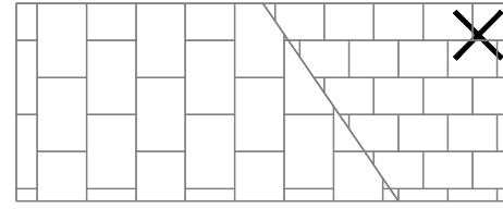
Cut edge of block pavers abuts different material. Cuts give small triangular pieces at material junction.
