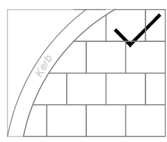
Inboard cuts using half pavers to avoid smaller pieces at kerb edge.
