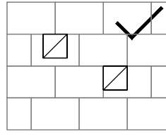
Cover abuts at least one whole paver, preferably two pavers.
