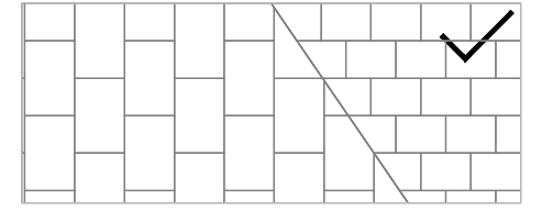
Block pavers laid to form parallel edge to different material. Block pavers laid and cut to give maximum block size at cut.
