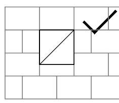
Cover abuts at least one whole paver, preferably two pavers.
