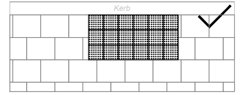
Whole and half pavers used at material junction.
