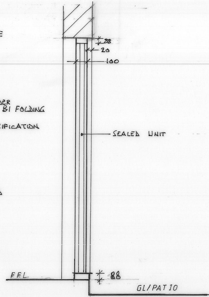
SECTION
