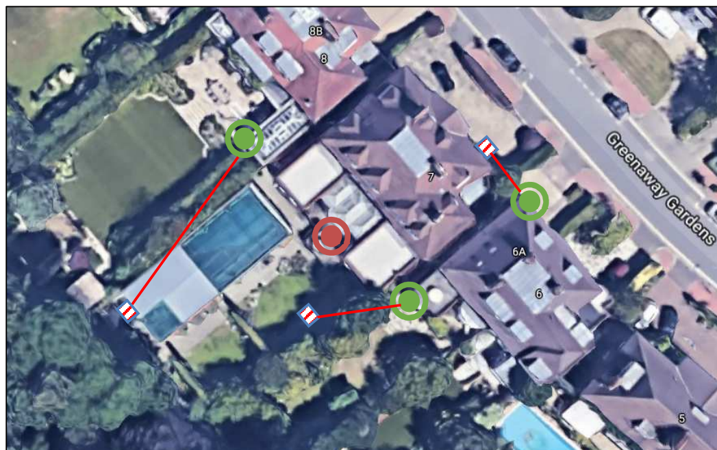
Figure 2.2 Site measurement position, identified receivers and proposed plant unit installations (Image Source: Google Maps)
