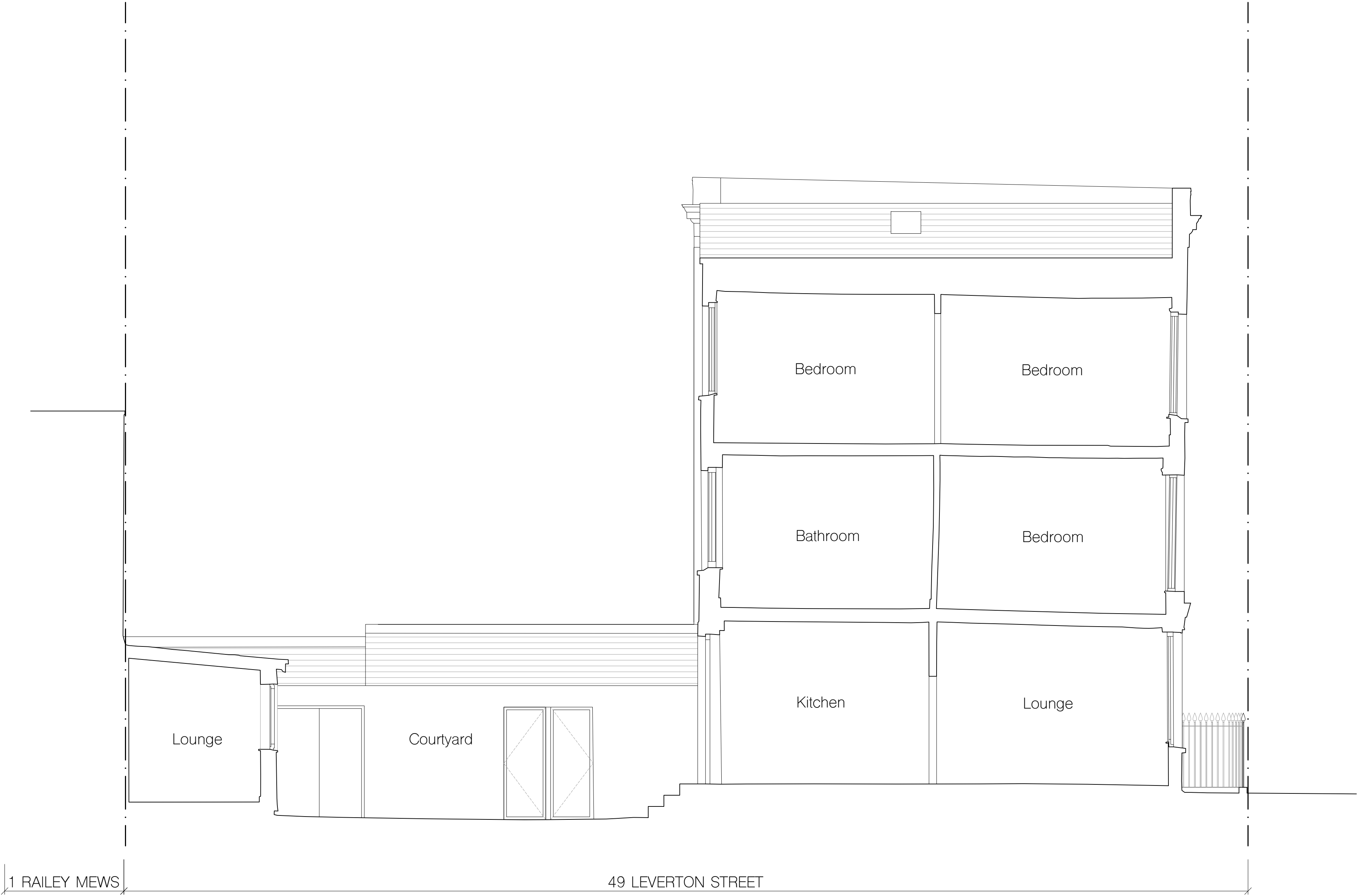
1 Existing section AA
