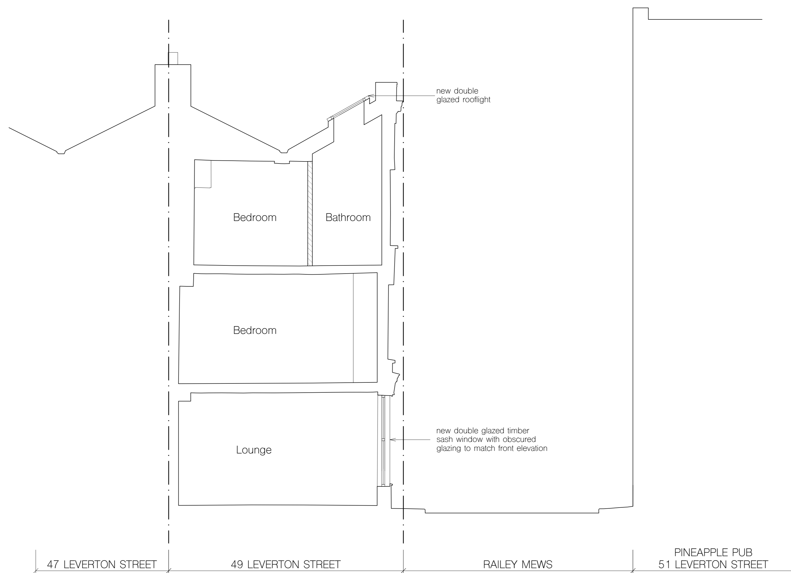
1 Proposed section DD
