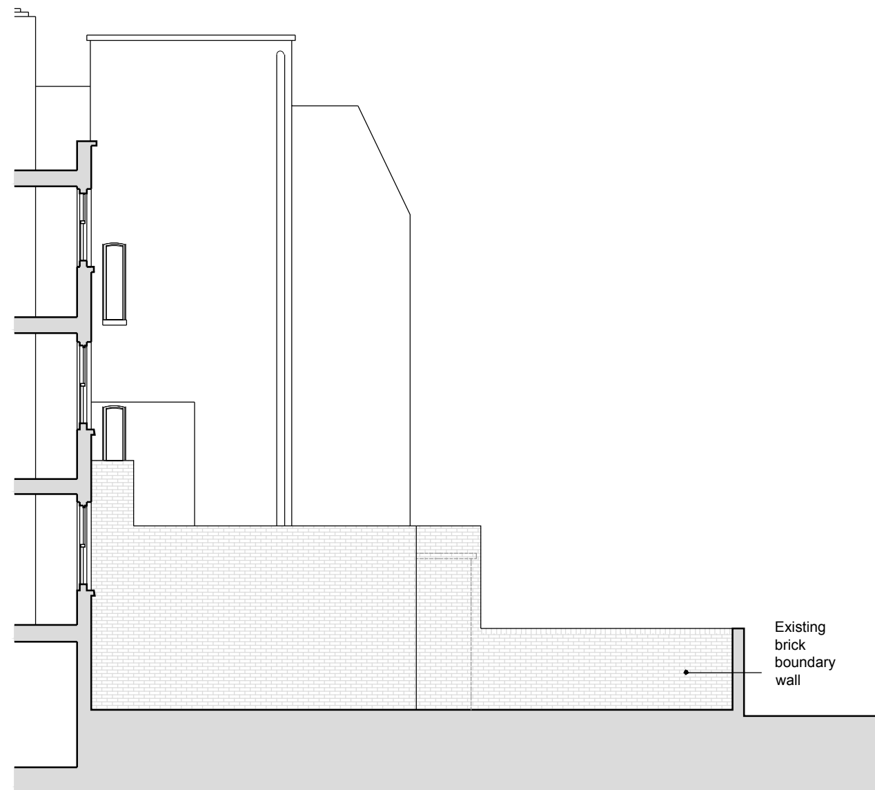
EXISTING ELEVATION 0 1 5m
