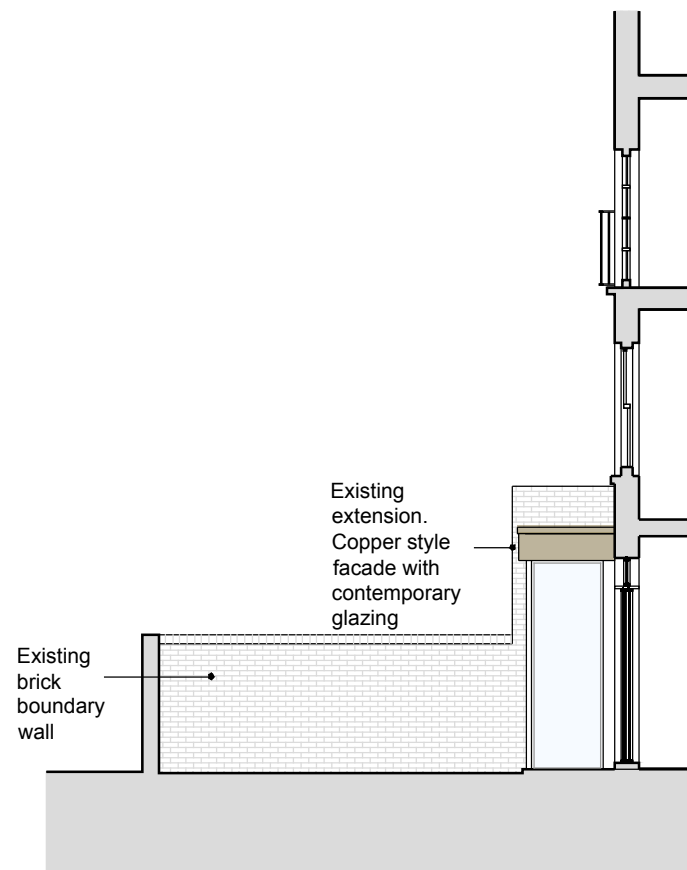
EXISTING ELEVATION 0 1 5m
