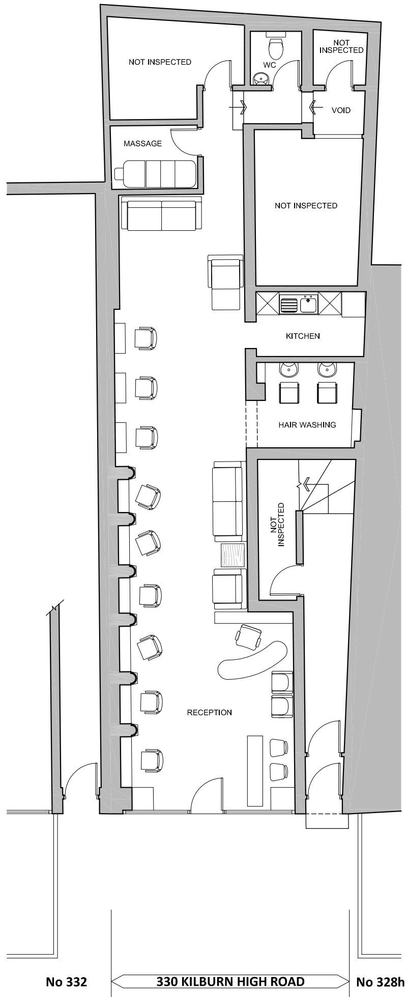
EXISTING GROUND FLOOR PLAN SCALE 1:100 @ A3
