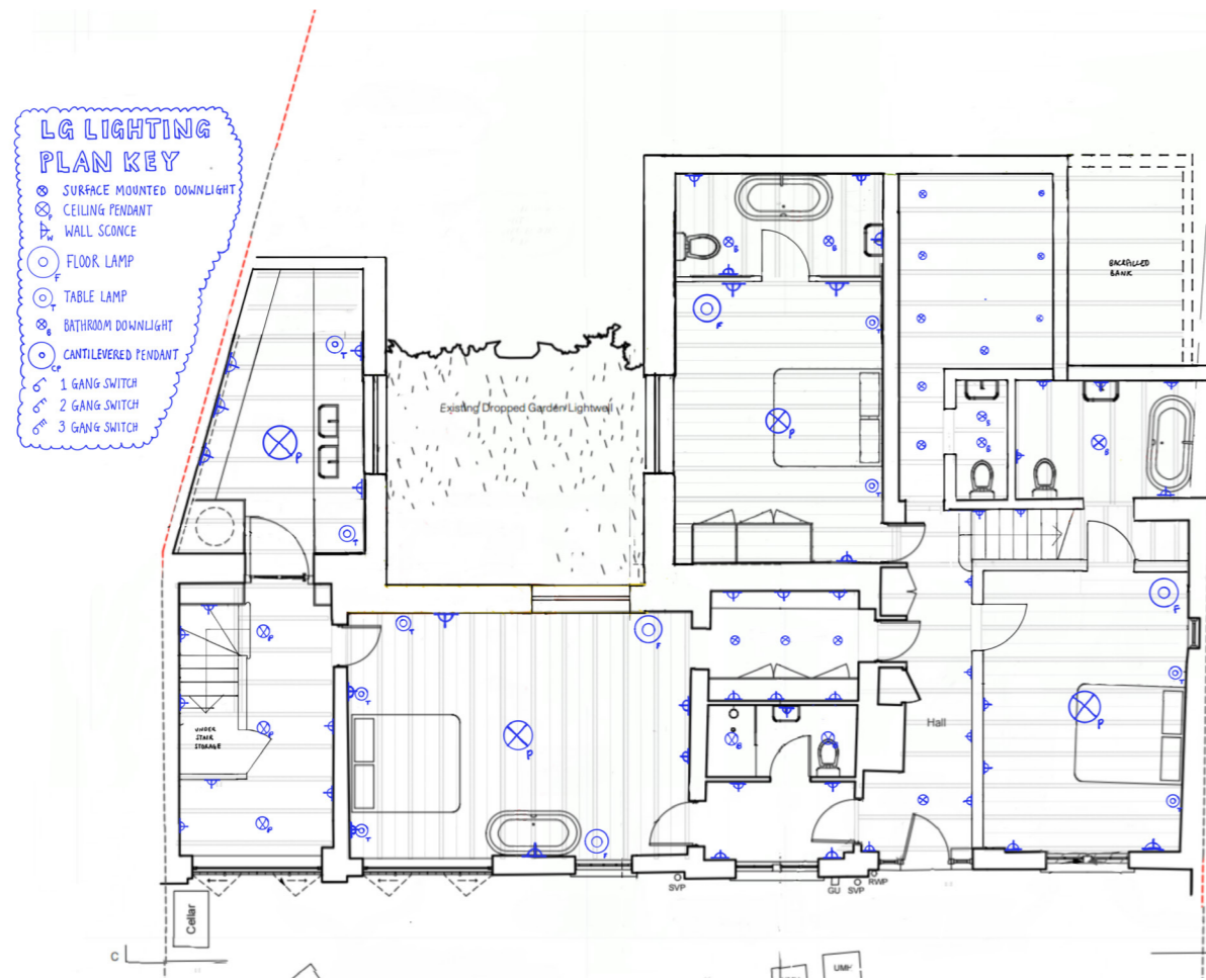
LG FLOOR LIGHTING PLAN
