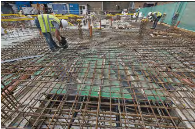
REINFORCED CAST IN SITU FLOOR SLAB
