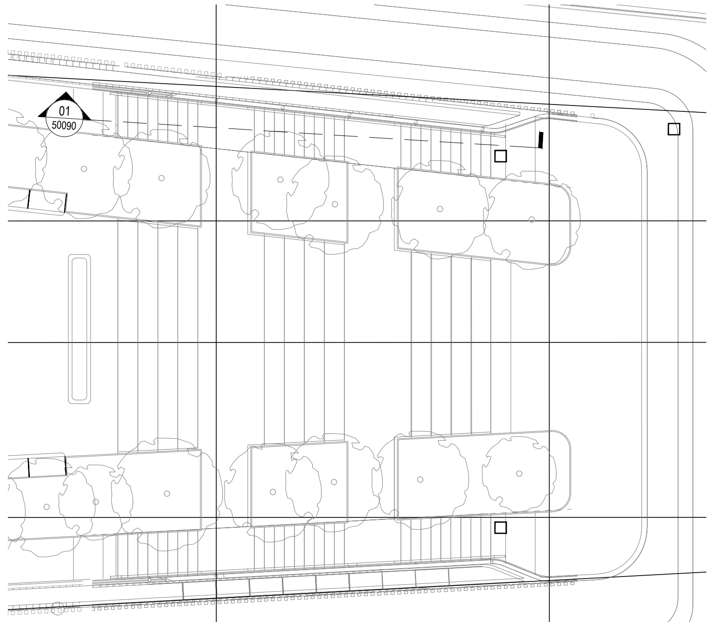
Headland plan Scale 1: 100 @ A0
