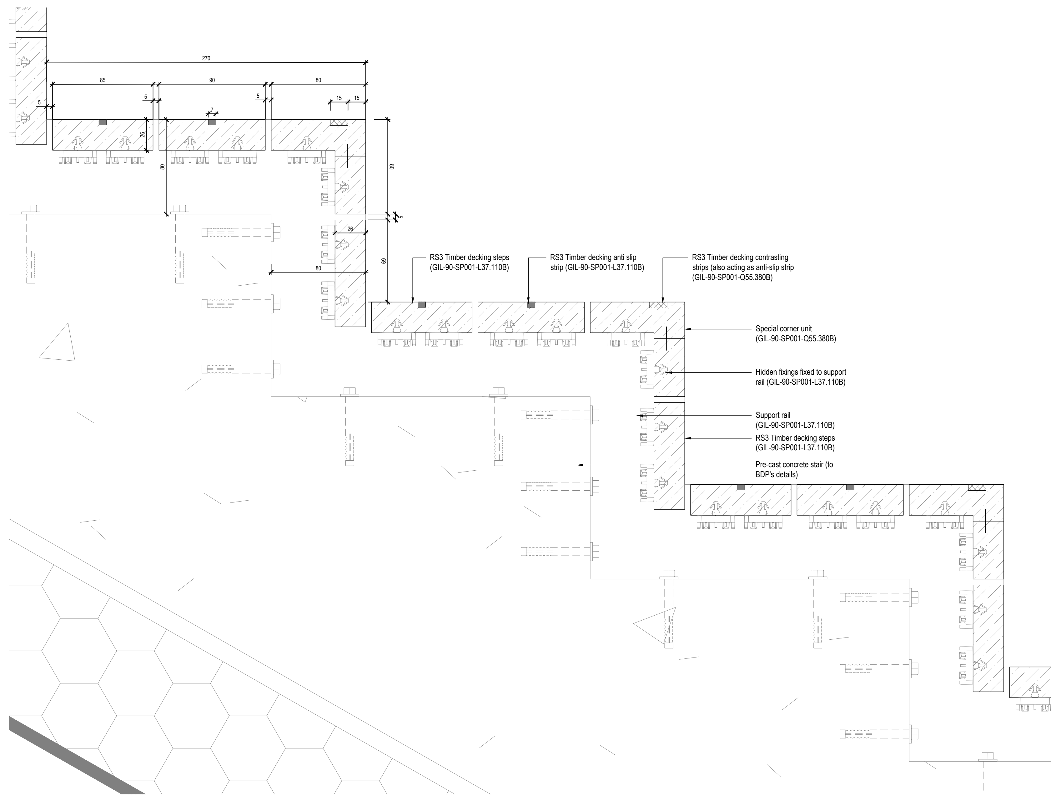
Headland Step 01 - Callout 01 Scale 1:2 @ A0
