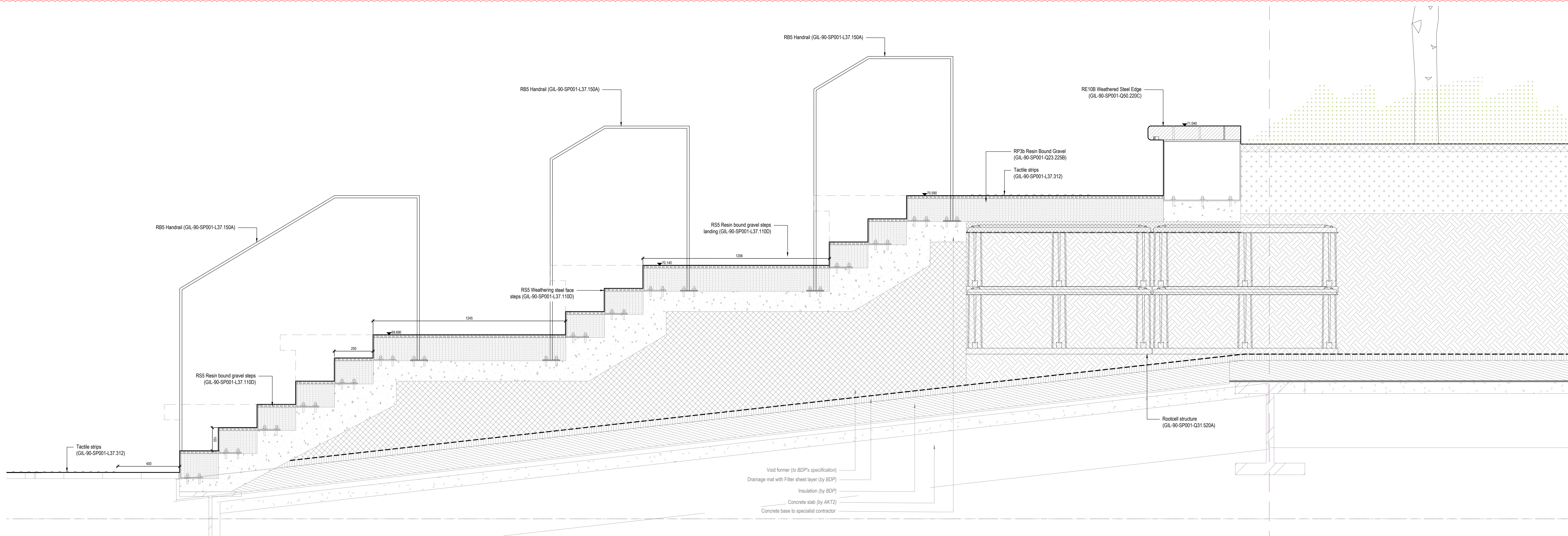
01 Plateau Amphitheatre detail - section 02 Scale 1:10 @ A0
