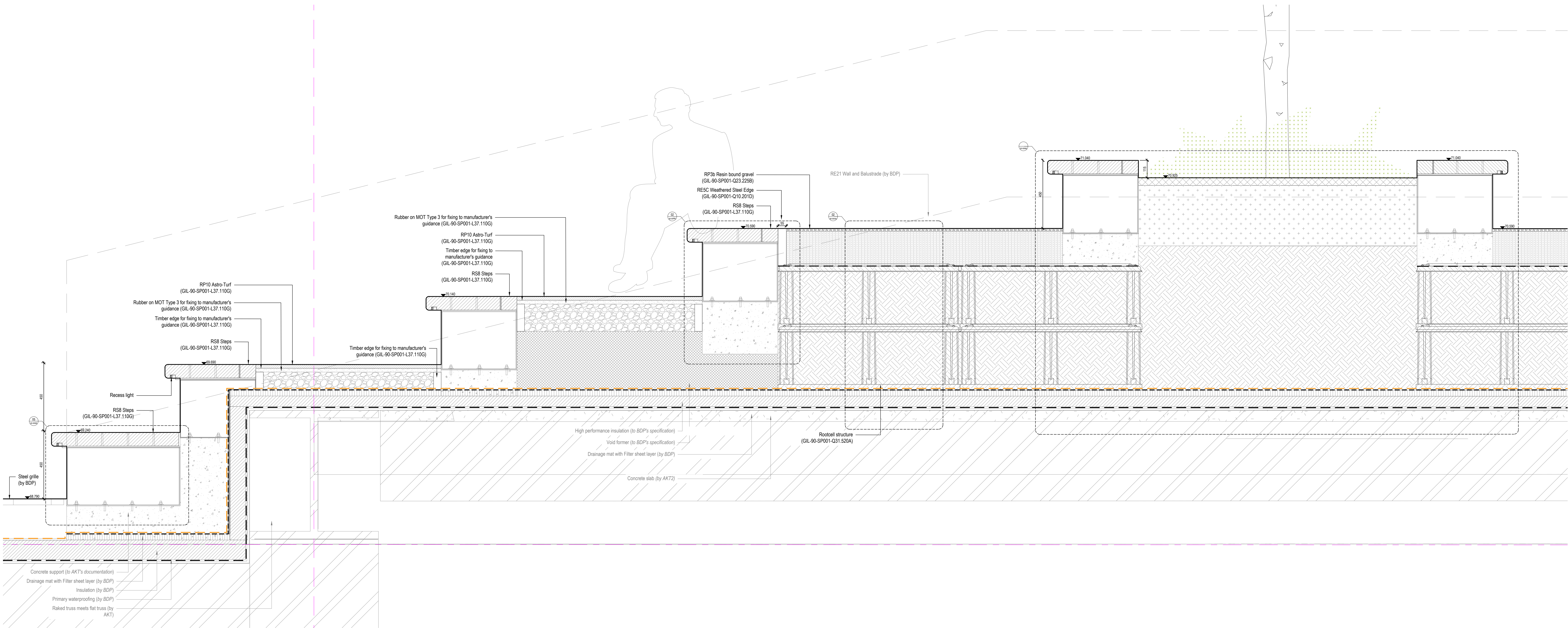
01 Plateau Amphitheatre detail - section 03 Scale 1:10 @ A0
