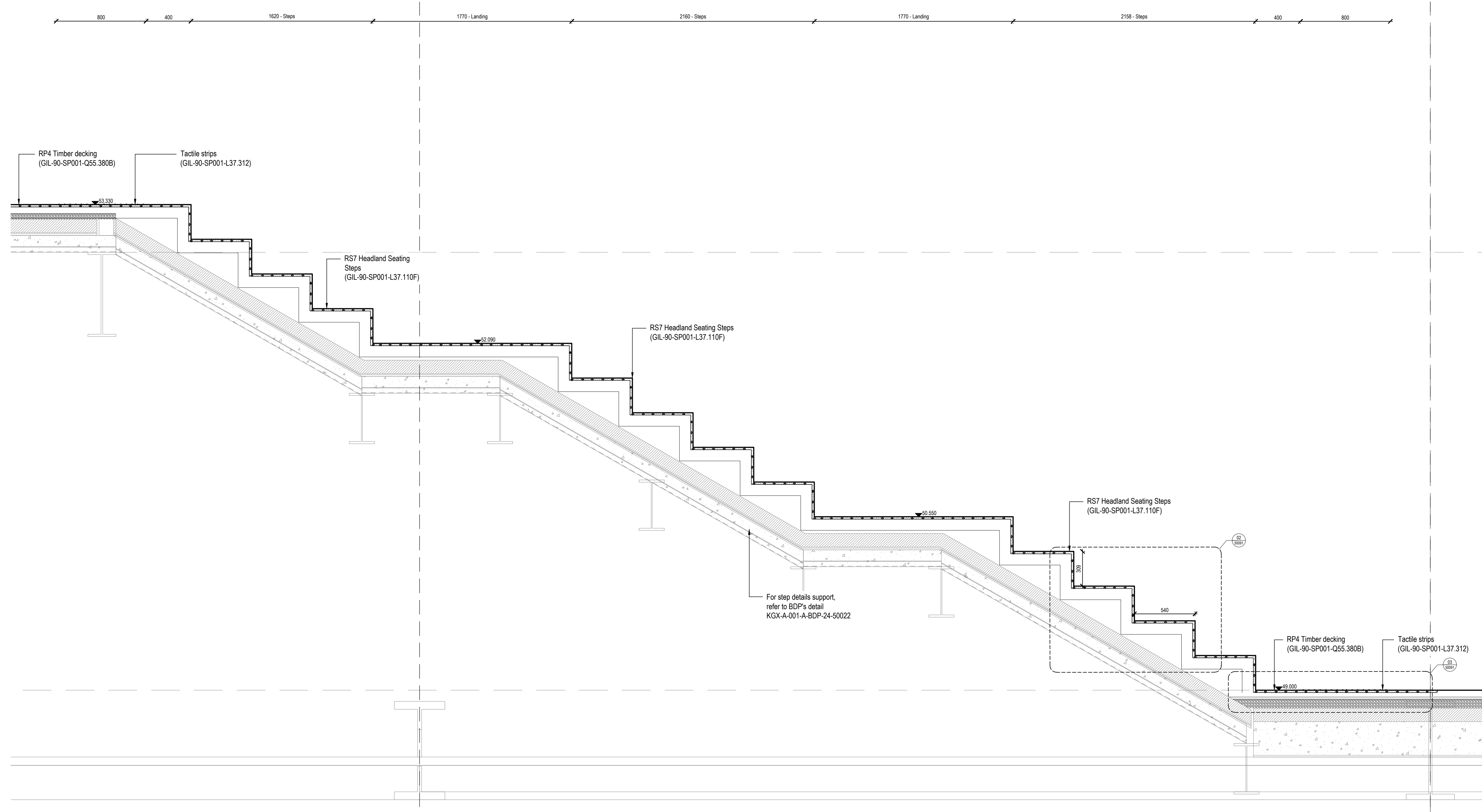
02 50096 Headland Amphitheatre detail 02 Scale 1:20 @ A0
