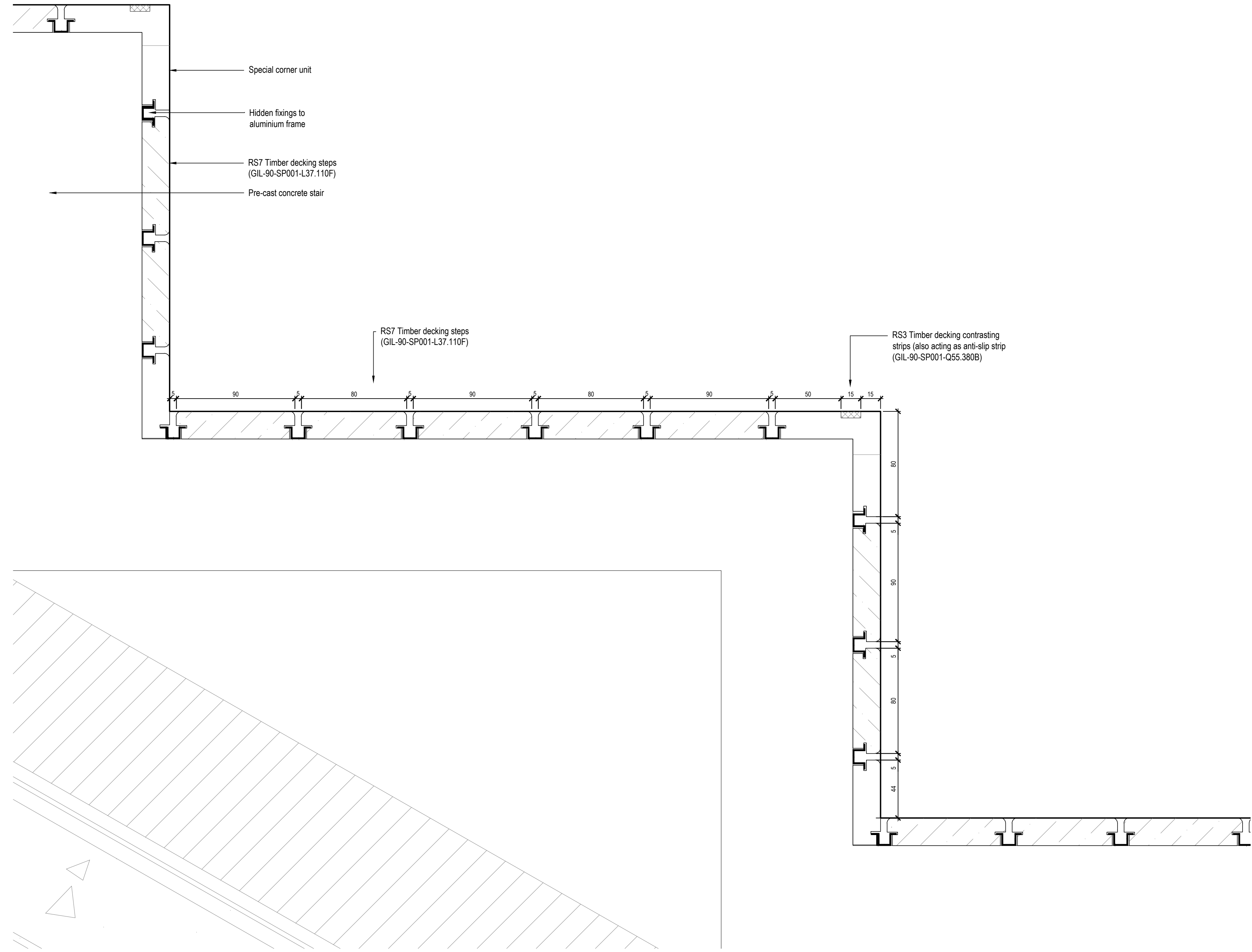
02 50097 Headland Amphitheatre detail 02 - Callout Scale 1:2 @ A0
