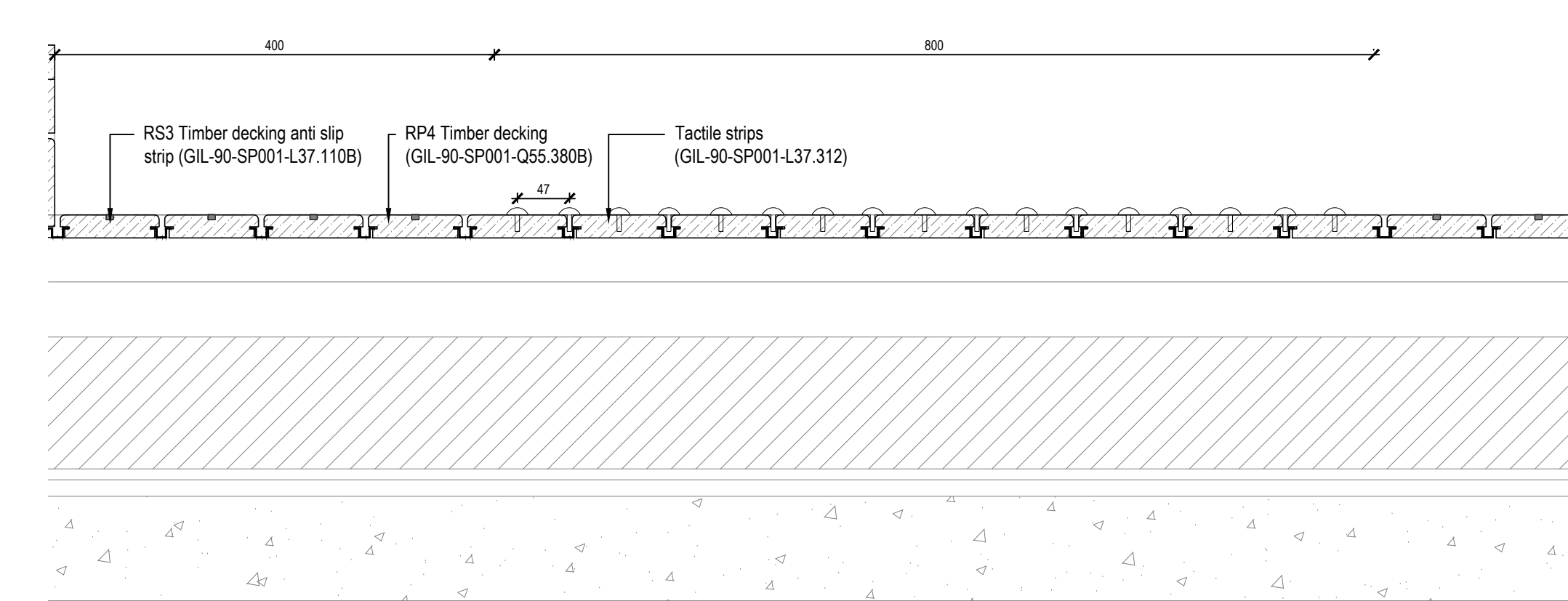
03 50098 Headland Amphitheatre detail 03 - Callout Scale 1:2 @ A0
